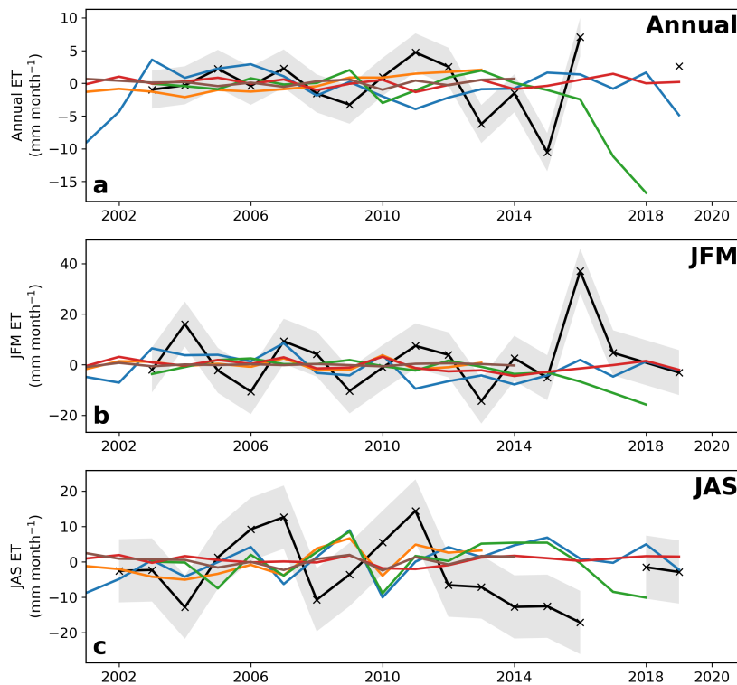
Fig. 1. Interannual variation in evapotranspiration from 2001 to 2019.
