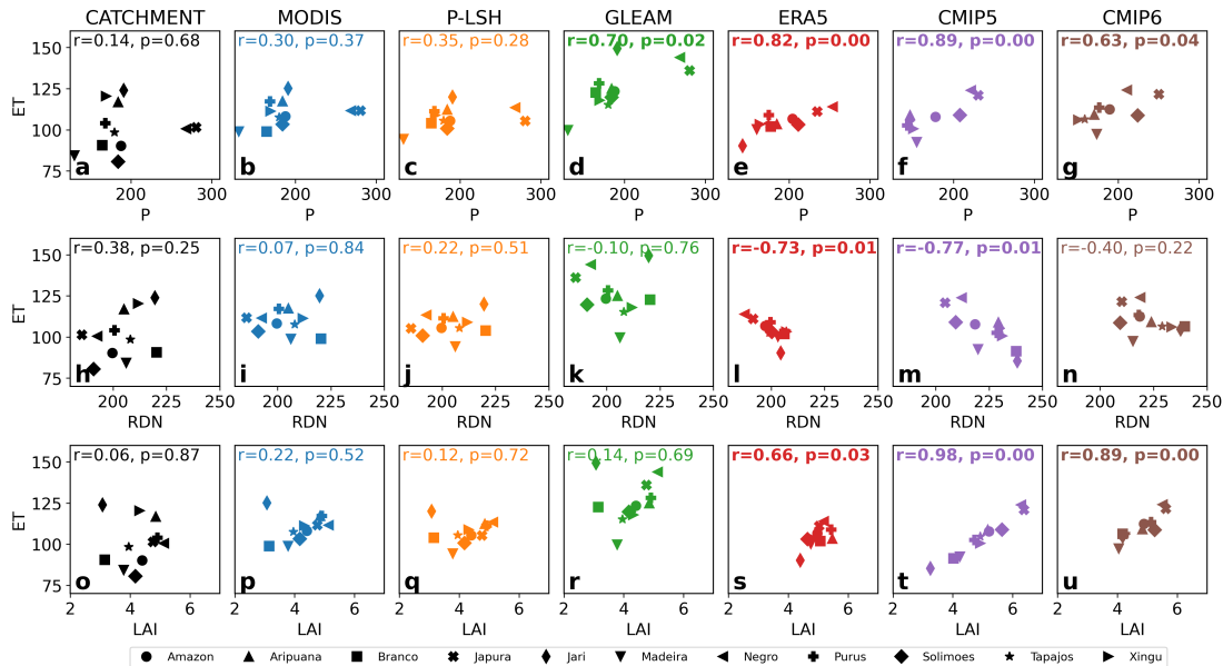
Fig. 3. Controls on spatial variation in Amazon evapotranspiration. Annual mean ET (in mm month -1 ) for the Amazon and ten sub-catchments (Fig. 1) from catchment-balance, satellites (MODIS, P-LSH, G
