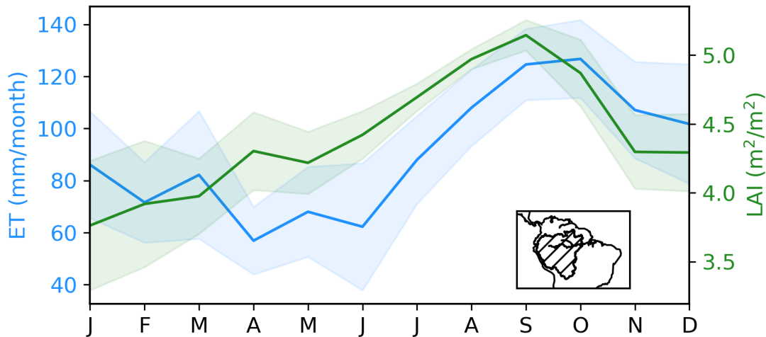
Fig. 2. Seasonal variation in leaf area index over the Amazon. Climatological seasonal cycles in catchment-balance ET (blue) and MODIS MOD15A2H Collection 6 LAI (green) averaged over the Amazon region shown i
