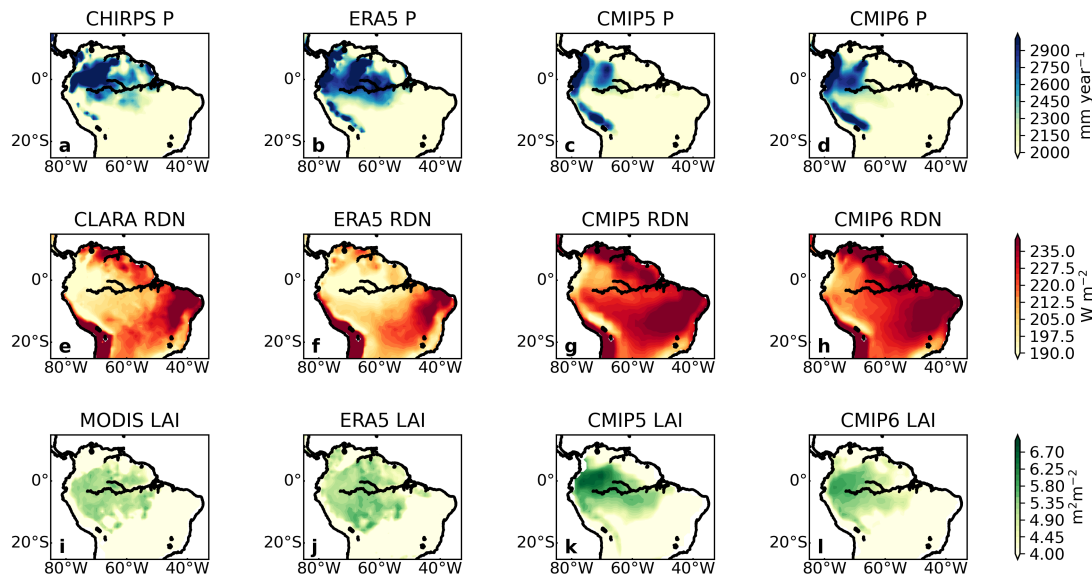
Fig. 1. Climatological annual precipitation, radiation and leaf area index. Mean annual precipitation (P, a–d), radiation (RDN, e–h) and leaf area index (LAI, i–l) from satellites (column 1), reanalysis (column 2), and climate models (columns 3 and 4).
