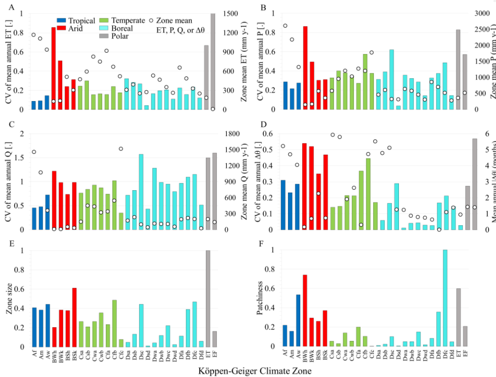
295 Figure 1: Water budget coherence, quantified as intra-zone CV (A-D), and complexity metrics of zone size and patchiness (E-F) for each zone for the Köppen-Geiger climate classification system. Mean hydroclimate values for each zone are also shown (circles, A-D). Zone size (number of pixels) and patchiness (number of patches) are normalized to their maximum values.
