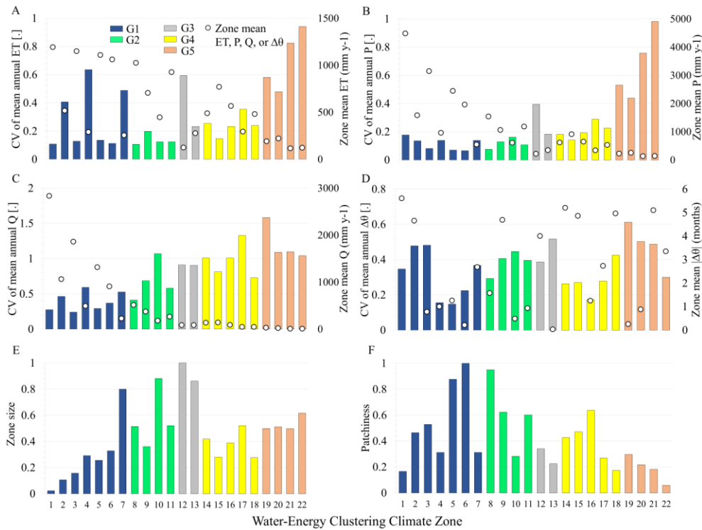
Figure 2. Water budget coherence (intra-zone CV, A-D) and complexity metrics (zone size and patchiness, E-F) for each zone for the Water-Energy Clustering (WEC) climate classification system. Mean hydroclimate values for each zone are also shown (circles, A-D). Zone size (number of pixels) and patchiness (number of patches) are normalized to their maximum values.
