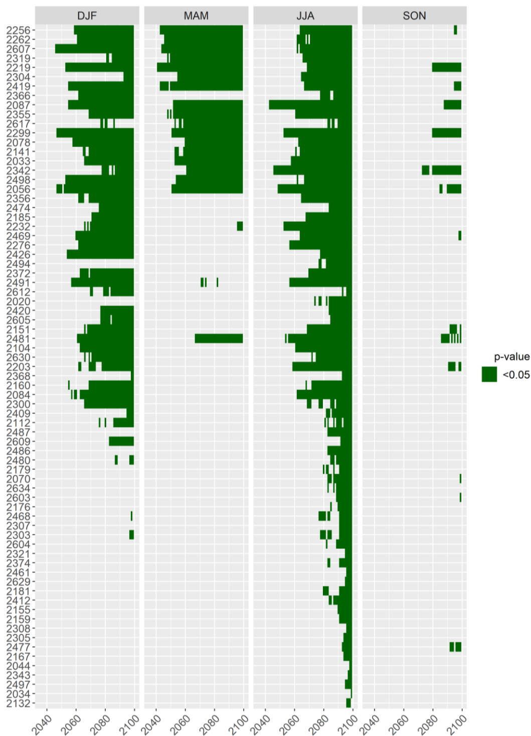
Figure 7: Temporal evolution of time of emergence for the different seasons. Periods where p-value of the Kolmogorov-Smirnov test is lower than 0.05 are highlighted. Only catchments with at least one detection of time of emergence in one of the seasons are shown. Catchments are ordered by mean altitude of the catchment with highest altitudes at the top.
