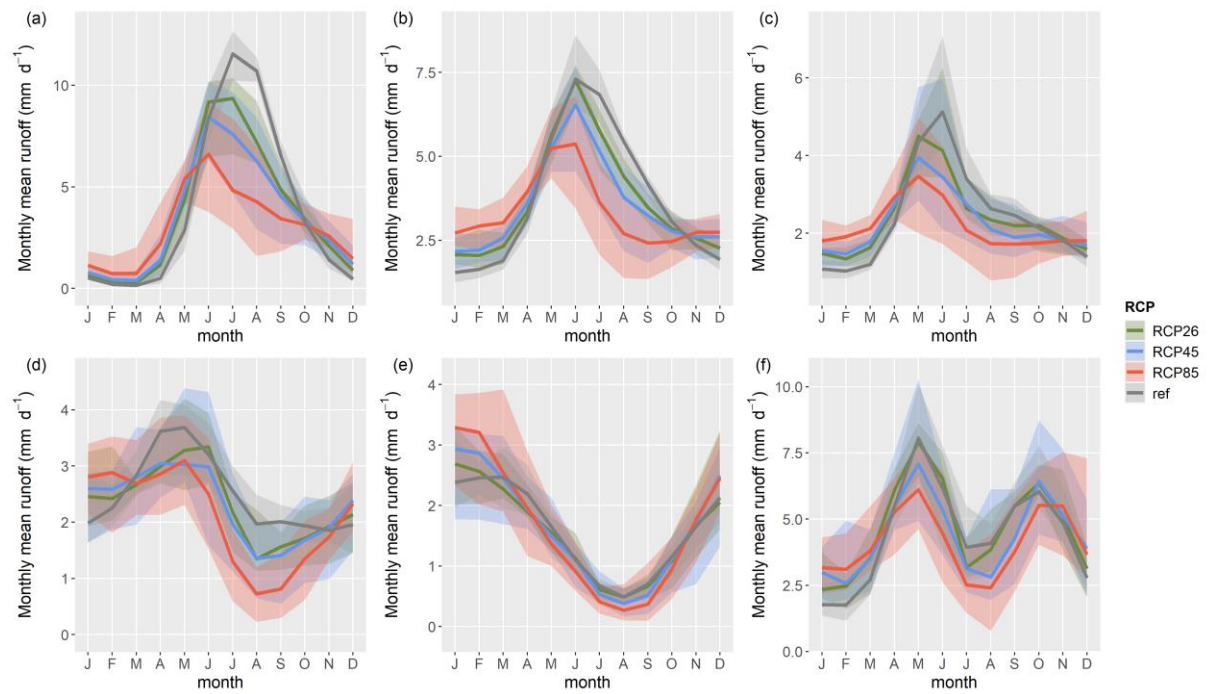
Figure S5: Runoff regimes for the six representative catchments Rosegbach (a), Kander (b), Plessur (c), Emme (d), Venoge (e), and Verzasca (f). Thick lines represent the multi-model median for the reference period (grey), for 2085 under RCP2.6 (green), for 2085 under RCP4.5 (blue), and for 2085 under RCP8.5 (red). Shadings show the full model range for each RCP.
