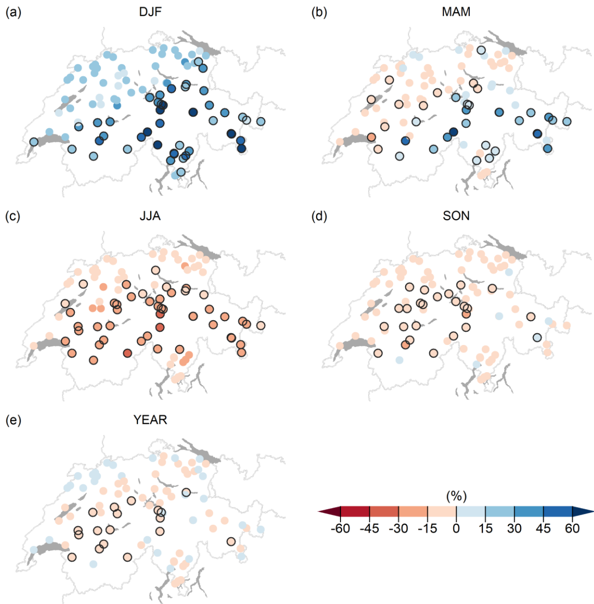
Figure S1: Multimodel median of seasonal and yearly mean changes under RCP4.5 by 2085 for winter (a), spring (b), summer (c), autumn (d), and yearly means (e). Black circles indicate changes with at least 90% of the models agreeing on the direction of change.
