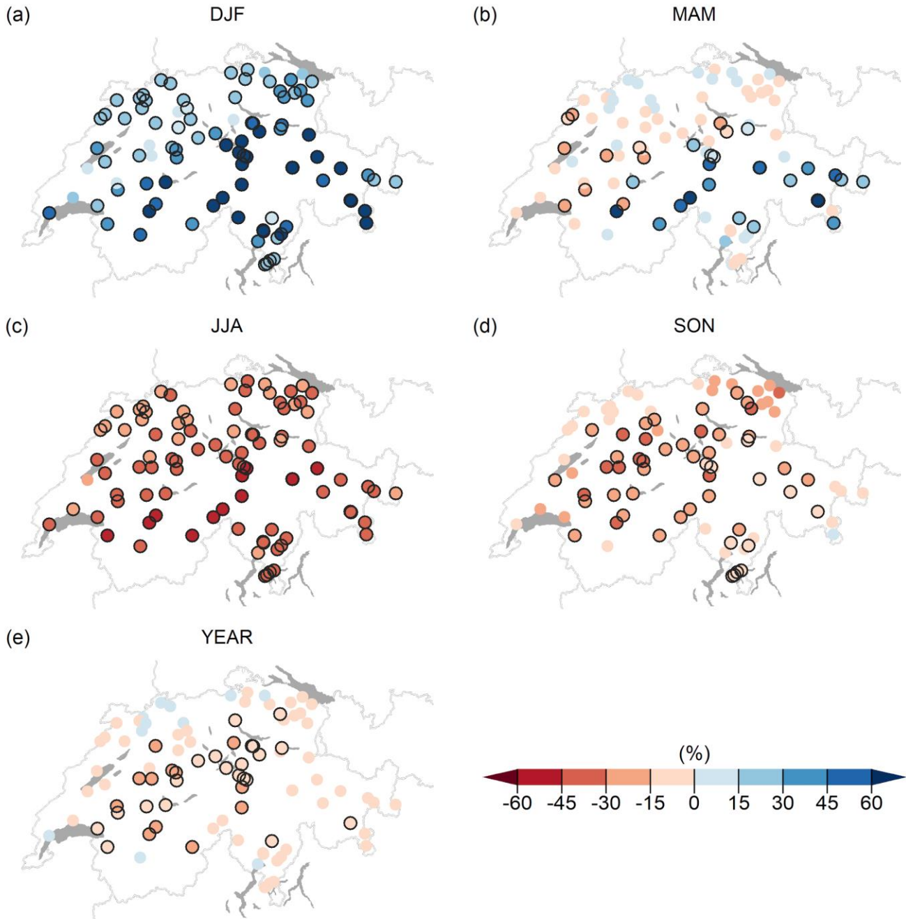
620 621 Figure 2: Multimodel median of seasonal and annual mean changes of runoff under RCP8.5 by 2070–2099 for winter (a), spring (b), 622 summer (c), autumn (d), and annual means (e). Black circles indicate catchments whose direction of change agrees across at least 623 90% the models.
