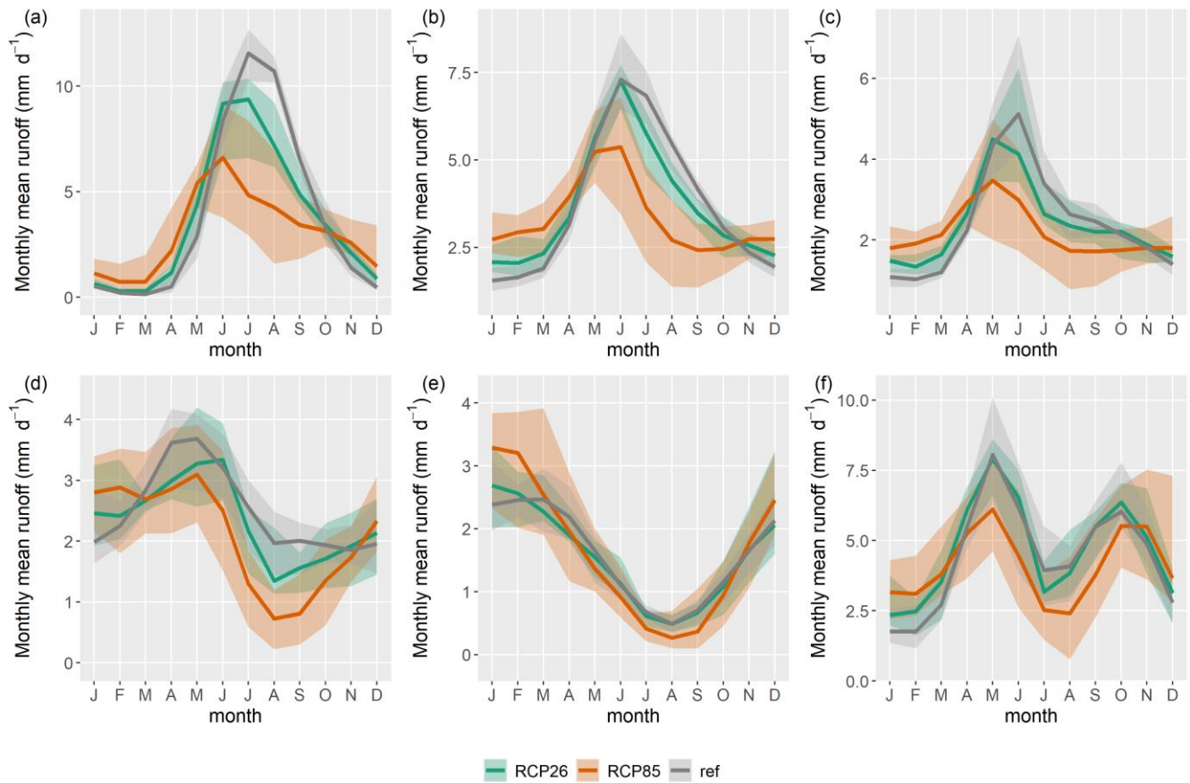
634 635 636 Figure 5: Runoff regimes for the six representative catchments: Rosegbach (a), Kander (b), Plessur (c), Emme (d), Venoge (e), and 637 Verzasca (f). Thick lines represent the multimodel median for the reference period (grey), for 2070–2099 under RCP2.6 (turquoise), 638 and for 2070–2099 under RCP8.5 (orange). Shadings show the full model range for each RCP.
