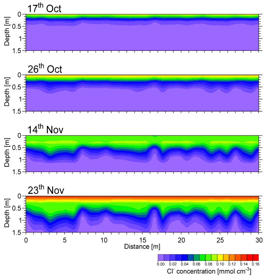
Figure 7: Soil Cl - concentration distributions simulations for the selected scenario: a) 17 Oct, b) 26 Oct, c) 14 Nov and d) 23 Nov 2016
