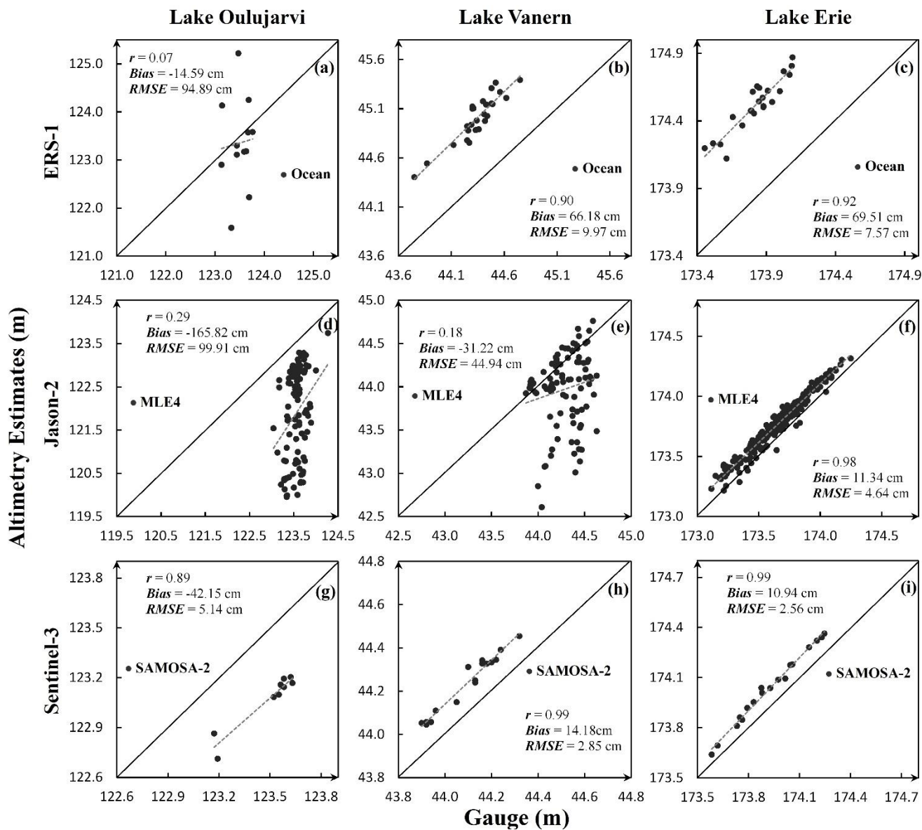
940 Figure 6. Scatterplots of lake water level estimates given by model-based retracers against gauge measurements. The scatterplots of the same mission are arranged in the row and the scatterplots of the same lake are arranged in the column.
