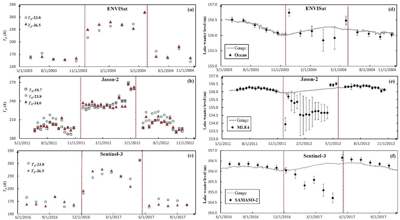
925 Figure 3. Time series of mean brightness temperature ( T_B ) and lake level estimates produced by ENVISAT, Jason-2 and Sentinel-3 over Great Slave Lake in the winters. (a) T_B in 2003/2004 winter, (b) T_B in 2011/2012 winter, (c) T_B in 2016/2017 winter, (d) lake level estimate in 2003/2004 winter, (e) lake level estimates in 2011/2012 winter; and (f) lake level estimates in 2016/2017 winter.
