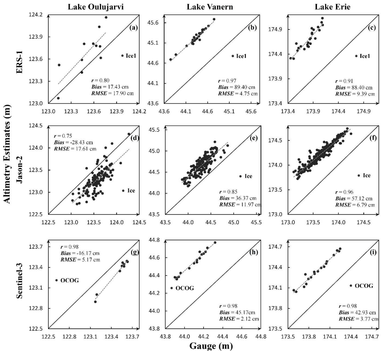
935 Figure 5. Scatterplots of lake water level estimates given by model-free retracers against gauge measurements. The scatterplots of the same mission are arranged in the same row and the scatterplots of the same lake are arranged in the same column.
