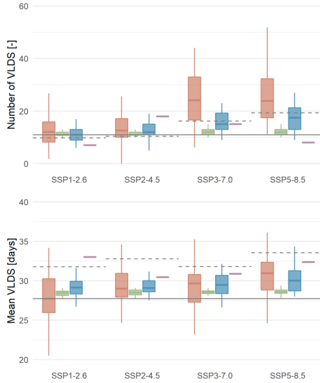
Figure 6. Boxplot representation of results for number of dry spells and dry spell length under different future scenarios. WG downscales the ensemble as a whole, resulting in only one data point. CMIP6 GCM projections (not downscaled; dashed line) and Uccle observations (solid line) are given as reference. VSDS, SDS, MDS, LDS and VLDS denote very short, short, medium, long and very long dry spells, respectively. Top and bottom of the box show the 75th and 25th percentiles of the relative error, respectively. Top and bottom of the whiskers show the 5th and 95th percentiles, respectively. Horizontal black line in the middle of the box represents the median.
