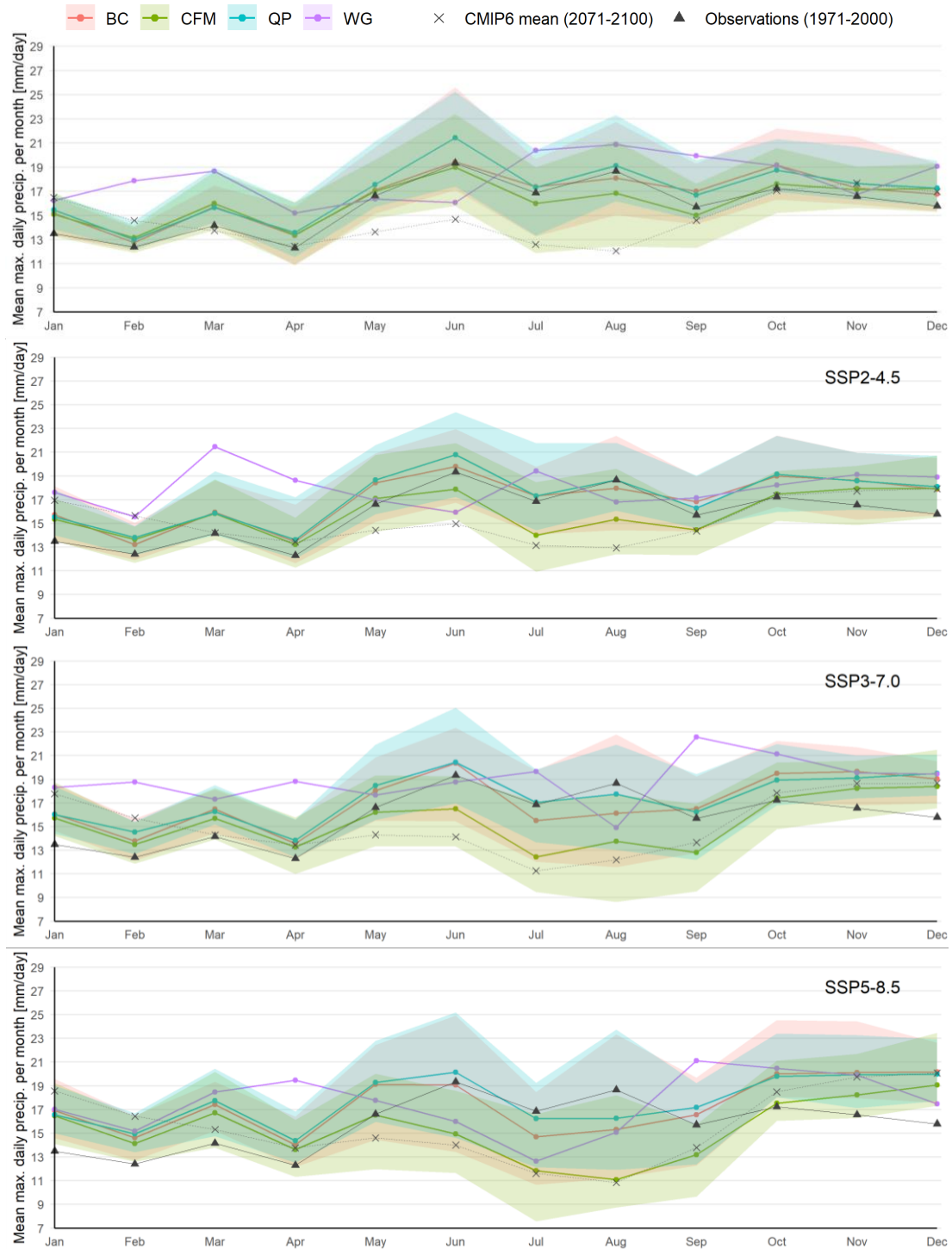
Figure 8. Graphical representation of results for maximum daily precipitation under different future scenarios. Coloured lines represent median values of the ensemble, shades represent the variation within the ensemble (10% – 90% quantiles). CMIP6 GCM projections (not downscaled; dashed line) and Uccle observations (solid line) are given as reference.
