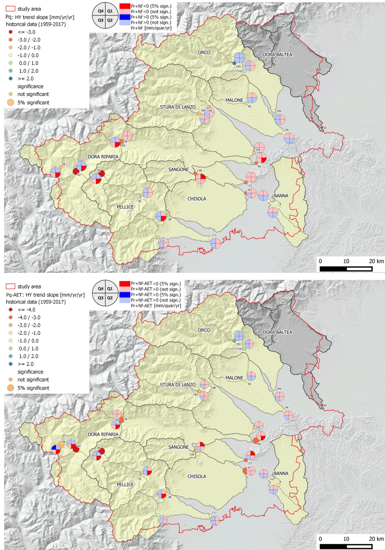
Figure 6. Trend slope at the catchment level for all studied catchments. Top: total precipitation, bottom: drainage. Hydrological year (full dots) and quarterly trend values (four-segments circles) are jointly represented, and trend significance is also indicated. When quarters are considered, the precipitation is the sum of liquid precipitation P_r and melted snow N_f . Topographic shading is based on DEM data from the Risknat Project
