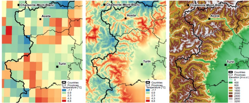
Figure 2. Maximum temperature field at (left) 0.125^\circ lon-lat spatial resolution from the original OI dataset and at (middle) 250 m resolution after interpolation with orographic correction, for January 1 st , 2009. The right panel shows the orography of the study area from a Digital Elevation Model derived from the SRTM project, interpolated at 250 m of spatial resolution.
