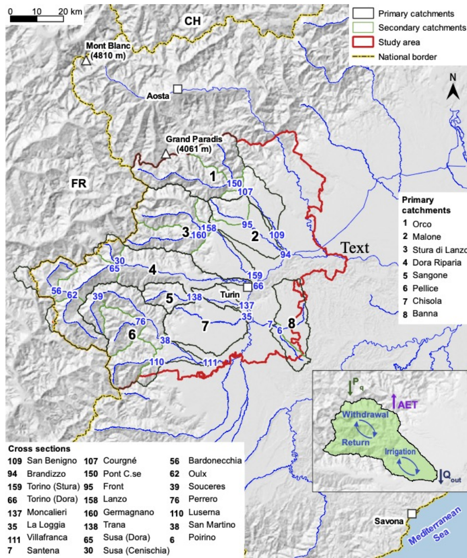
Figure 1. The study area including river catchments and sub-catchments. Illustration of the water balance terms at the catchment scale is shown in a bottom right box
