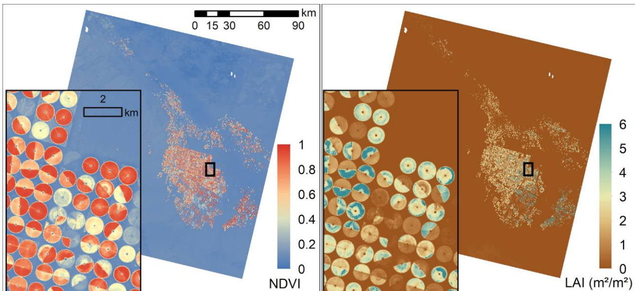
5 Figure 3: Example of the full Landsat tile (path/row 172/39) NDVI (left) and LAI (right) estimation, demonstrating the foot-print from center-pivot irrigated fields in this region (high contrast with the bare desert soil).
