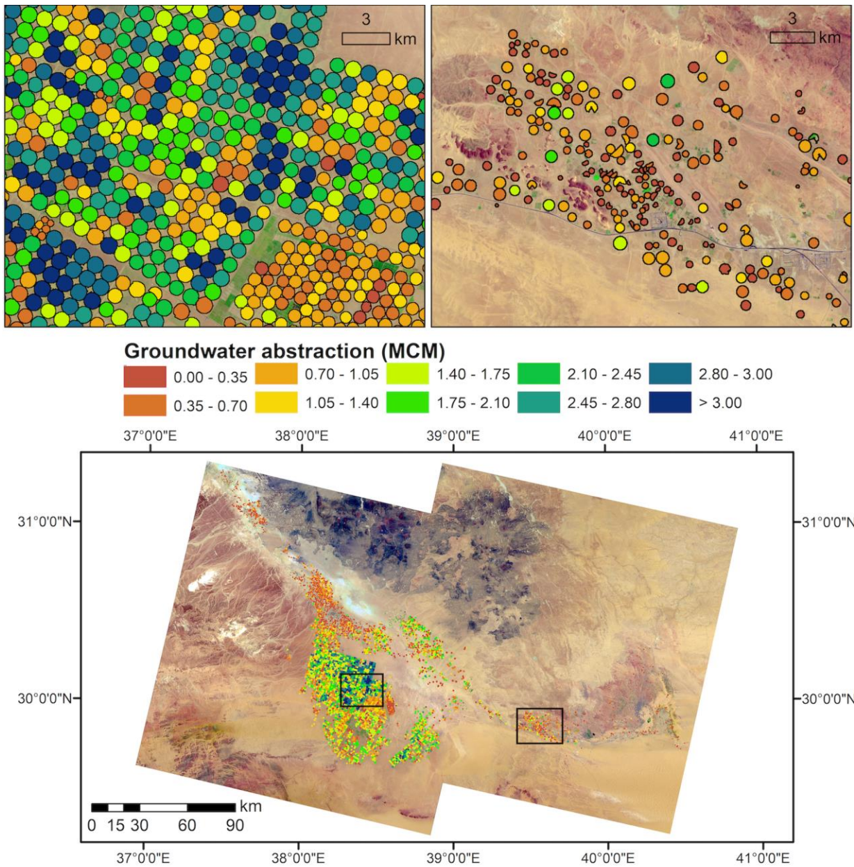
5 Figure 11: Map of annual groundwater abstraction in million cubic meters (MCM) for the Al Jawf agricultural region. Values were obtained for individual fields, as seen on the examples shown at top featuring one zone with high levels of abstractions (top-left) and another zone with a smaller density of fields and lower values of abstraction (top-right). The background shows the same Landsat 8 images as in Fig. 2.
