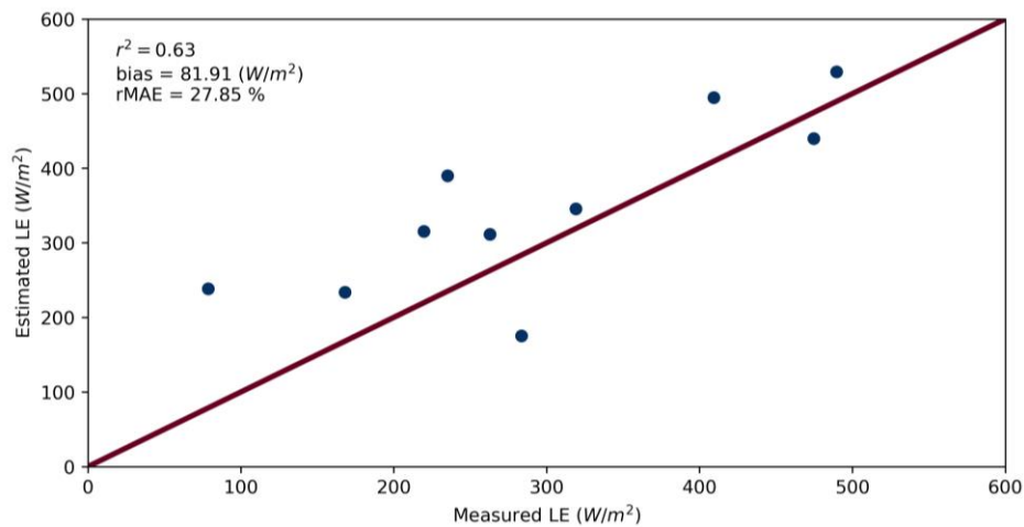
Figure S2: Evaluation scatterplot of measured vs. estimated LE fluxes using the series-TSEB model approach over an irrigated maize field (Tawdeehiya farms) in 2016.
