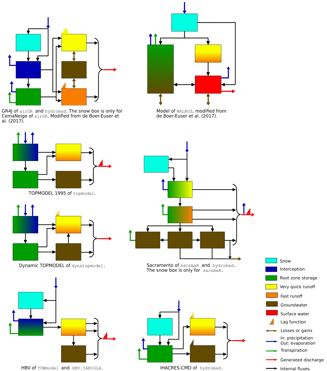
Figure 1. Unified diagrams illustrating the depiction of conceptual storages and fluxes by the main models contained in the selected packages. The root zone storage usually corresponds to the soil moisture accounting or production function. Groundwater accounts for saturated soil zones and shallow aquifers involved in the catchment response. Fast runoff is similar to lateral flow or interflow. Bi-coloured rectangles are for two storages/fluxes modelled by the same store or by the same function simultaneously. Please note that for the semi-distributed models, the schemes only contain the storages and fluxes calculated on a single spatial unit.
