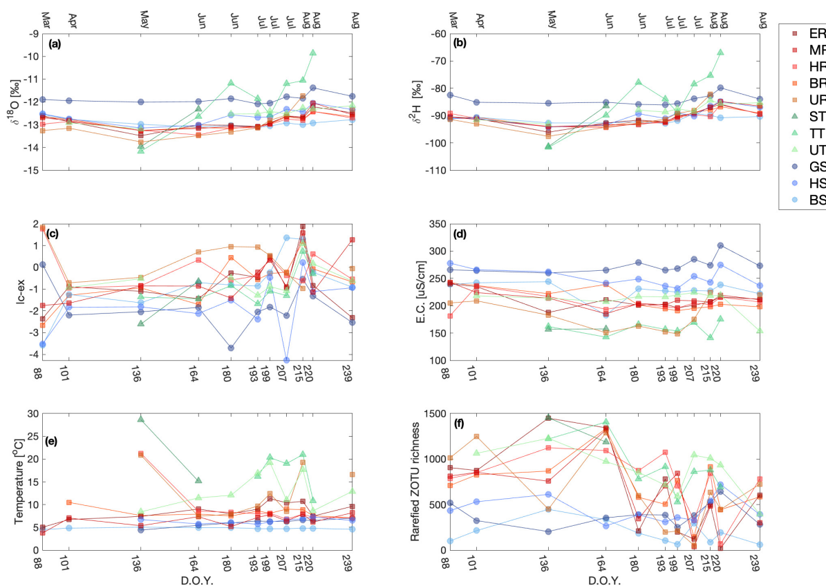
Figure 3. Variation in \delta^{18}\text{O} (a), \delta^2\text{H} (b), ic-ex (c), E.C. (d), temperature (e), and rarefied ZOTU richness (f) for the individual sampling sites over the field season (given as day of the year). The sampling sites in the legend are clustered based on the water source and within the cluster ordered from low to high elevation. The figure legend corresponds exactly to that in Fig. 1 and the x-axis corresponds exactly to that in Fig. 2.
