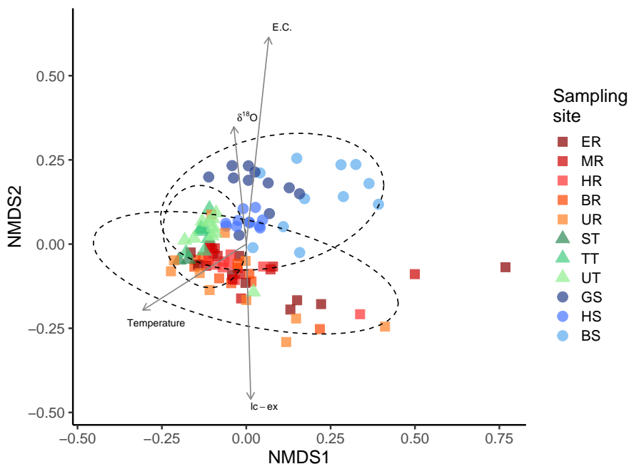
Figure 4. Community composition in the main channel, tributaries, and springs. Non-metric multidimensional scaling analysis of communities based on UniFrac dissimilarities (stress = 0.132, indicating a fair representation of the data in the reduced dimensions). Ellipses represent a 95% confidence interval.
