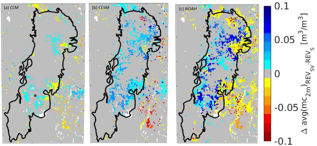
Figure 7. Difference between yearly averaged 2 m moisture content ( mc_{2m} ) of REV_{sv} and REVs in 2015, for (a-b-c) CLM, CLSM and NOAH, respectively. Blue colors highlight wetter soils after deforestation. The red dot in (a) represents the location of the time series shown in Figures 6 and 13.
