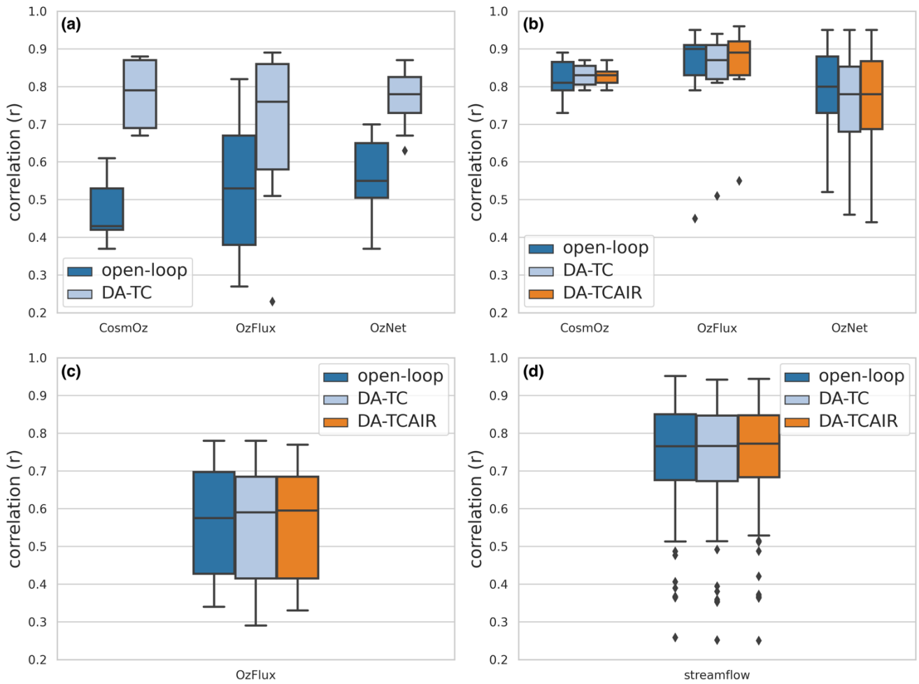
681 Figure 7: Distribution of correlation statistics of AWRA-L water balance estimates against in-situ measurements of (a) surface soil 682 moisture, (b) root-zone soil moisture, (c) evapotranspiration and (d) streamflow.
