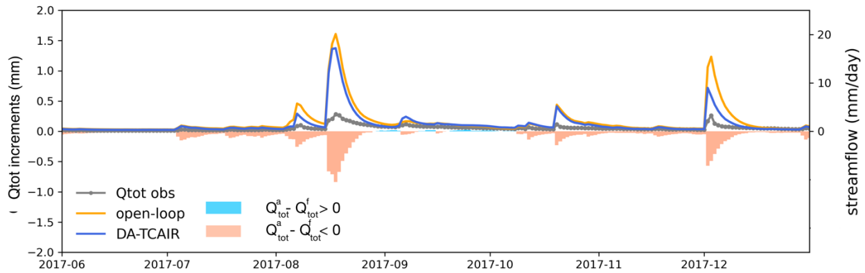
695 Figure 8: Changes in streamflow Q_{tot} estimates after the analysis increments redistribution (DA-TCAIR) for a catchment in south- 696 eastern Australia (centre coordinates: 36.63°E, 147.43°S) compared to in-situ streamflow observations ( Q_{tot} obs) and model open- 697 loop.
