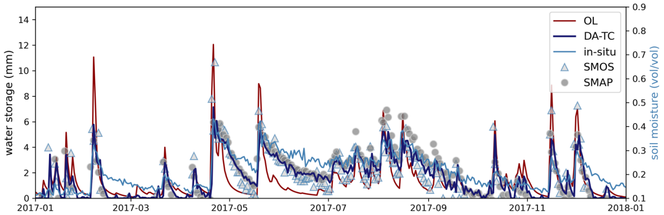
661 Figure 3: Time series of AWRA-L surface soil water storage estimates from open-loop (OL) compared to estimates after data 662 assimilation (DA-TC) of SMAP and SMOS soil moisture retrievals at CosmOz monitoring site: Bennets (35.826°E, 143.004°S). Note 663 that the in-situ soil moisture values are in volumetric unit.
