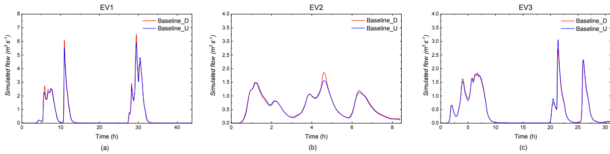
Figure 10: Simulated flow ( m^3 s^{-1} ) of the baseline scenario under three distributed rainfall events and three uniform rainfall events: (a) EV1, (b) EV2, (c) EV3.
