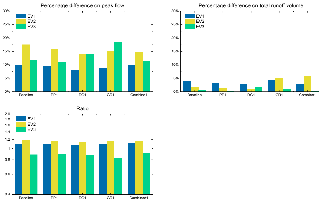
Figure 12. (a) Percentage difference on peak flow of the baseline scenario and the first set of NBS scenarios under the three distributed rainfall events and the three uniform rainfall events. (b) Percentage difference on total runoff volume of the baseline scenario and the first set of NBS scenarios under the three distributed rainfall events and the three uniform rainfall events. (c) The ratio of peak flow between the scenarios under the distributed rainfall and the scenarios under the uniform rainfall.
