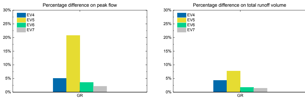
Figure 3A. (a) Percentage difference on peak flow of GR scenarios under the four syntactic rainfall events. (b) Percentage difference on total runoff volume of GR scenarios under the four syntactic rainfall events.
