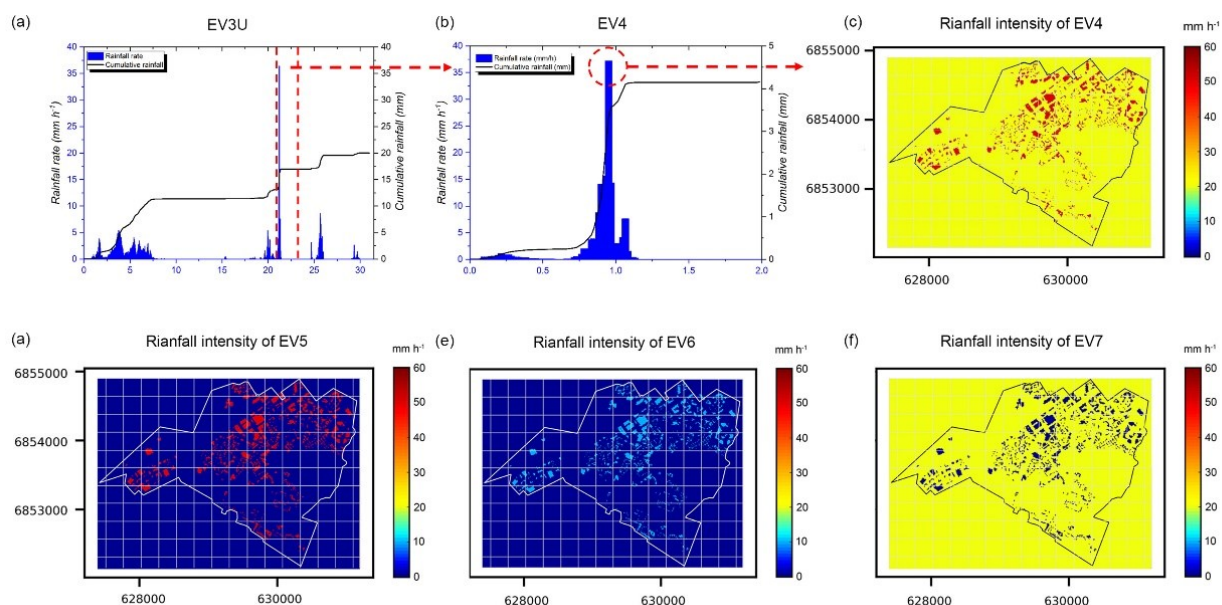
Figure. 1A (a) Time evolution of rainfall rate ( \text{mm h}^{-1} ) and cumulative rainfall (mm) of the EV3U over the whole catchment (the period between the red dash lines is the selected period for creating the EV4). (b) Time evolution of rainfall rate ( \text{mm h}^{-1} ) and cumulative rainfall (mm) of the EV4 over the whole catchment (the rainfall grid of rainfall peaks are modified based on the locations of GRs in GR1 scenario). (c) The rainfall intensity at the largest rainfall peak (gridded) over the Guyancourt catchment area for the EV4 (the red areas are the location of GRs in GR1 scenario with the highest rainfall intensity in space), the rainfall of other areas are uniform. (d) The rainfall intensity at the largest rainfall peak (gridded) over the Guyancourt catchment area for the EV5. (e) The rainfall intensity at the largest rainfall peak (gridded) over the Guyancourt catchment area for the EV6. (e) The rainfall intensity at the largest rainfall peak (gridded) over the Guyancourt catchment area for the EV7.
