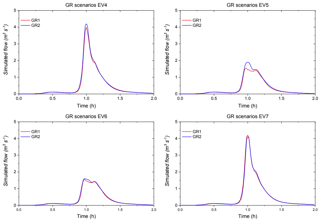
Figure 2A. Simulated flow ( \text{m}^3 \text{s}^{-1} ) of GR1 and GR2 scenario under the four syntactic rainfall events.
