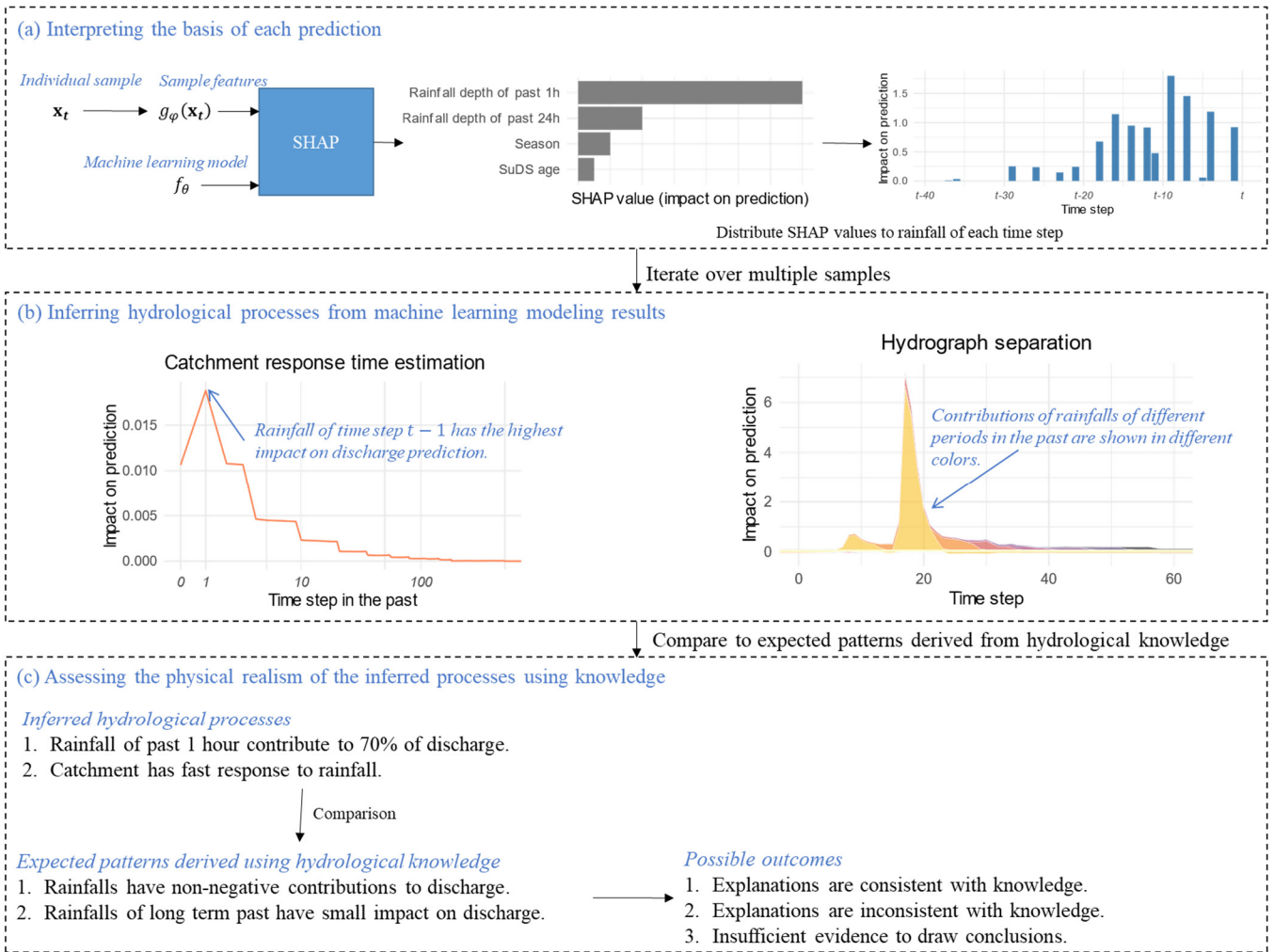
Figure 3 (a) Illustration of the processes for quantifying the contribution of each feature of an input sample x_t and distributing the contribution to the rainfall of each time step. (b) Examples of inferring the hydrological processes being modeled based on the basis of each prediction. (c) Examples of comparing the inferred hydrological processes to the processes expected based on the domain-specific knowledge of the system being modeled.
