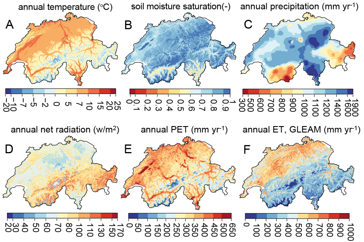
338 Figure 1. Spatial distribution of input data for the year 2004 at 500-m resolution: Annual mean (A) temperature 339 ( ^{\circ}\text{C} ), (B) soil moisture saturation (-, simulated by the PREVAH hydrological model), (C) precipitation ( \text{mm yr}^{-1} ), 340 (D) net radiation ( \text{W m}^{-2} ), (E) potential evapotranspiration (PET, \text{mm yr}^{-1} ) using the Priestley-Taylor equation 341 (Eq. 3), and (F) evapotranspiration (ET, \text{mm yr}^{-1} ) using the approach used in the GLEAM model (Eq. 1). See 342 Table. S1 for references.
