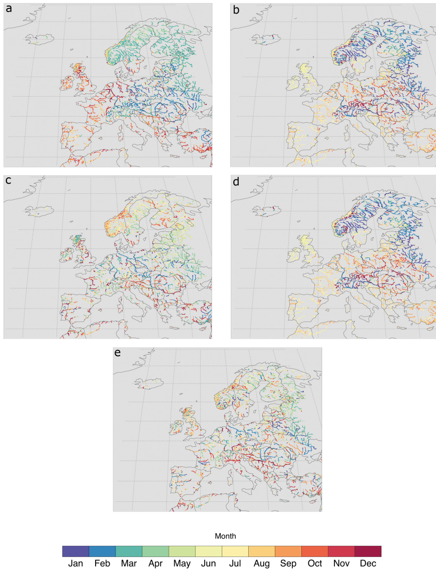
Figure 3. Drought timing (onset) in the European rivers from October 1990 to September 2018 identified using different drought identification methods: a) the VTD drought, b) the FTD drought, c) the VTM drought, d) the FTM drought, and e) the SSI-1 drought. For an explanation of the acronyms, see Fig. 2.
