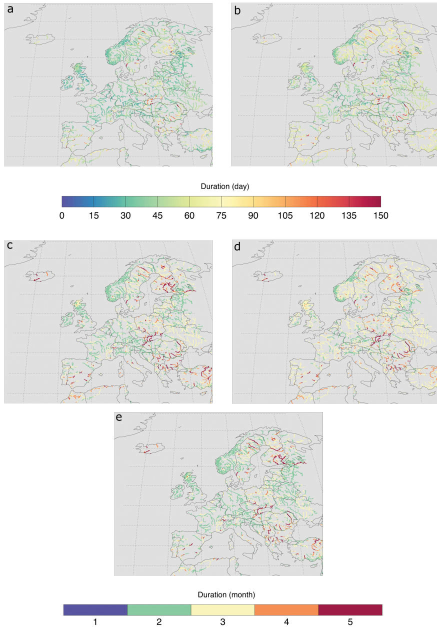
Figure B2. Average duration of drought events for the European rivers from October 1990 to September 2018 identified using different drought identification methods: a) the VTD, b) the FTD, c) the VTM, d) the FTM, and e) the SSI-1 approaches. For an explanation of the acronyms, see Fig. 2.
