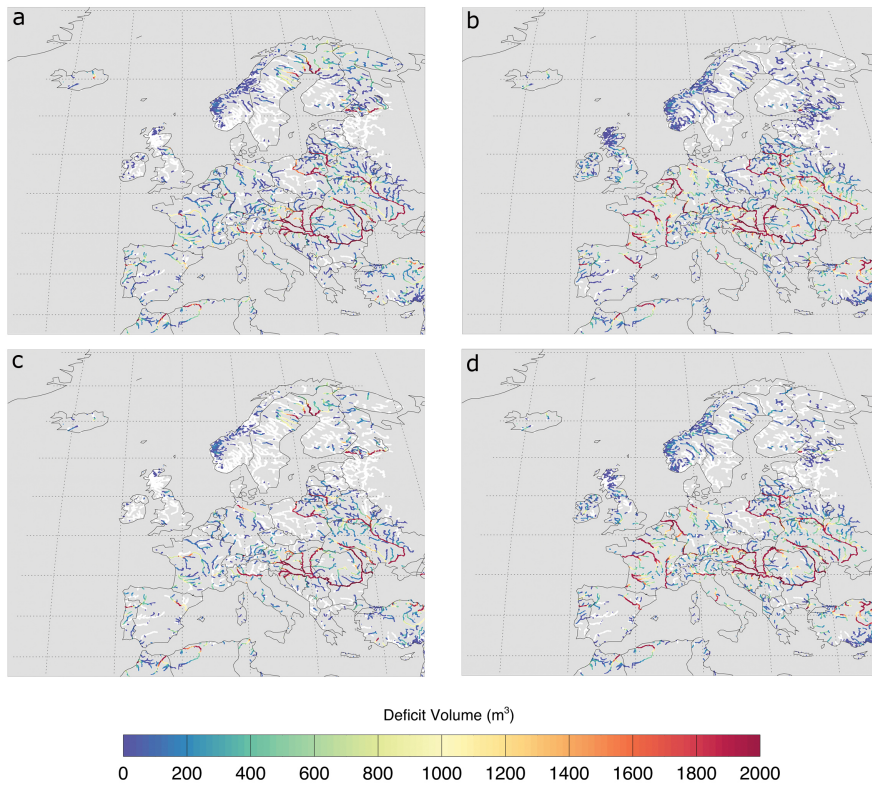
Figure C2. Forecasted average drought deficit volume (median of 25 ensemble members) in the European rivers using different drought identification methods and the forecast initiated on 1 st July 2003 with a lead time 7-month for: a) the VTD, b) the FTD, c) the VTM, d) the FTM, and e) the SSI-1 approaches. White river color indicates that no drought was forecasted. Note that deficit volume is not standardized.
