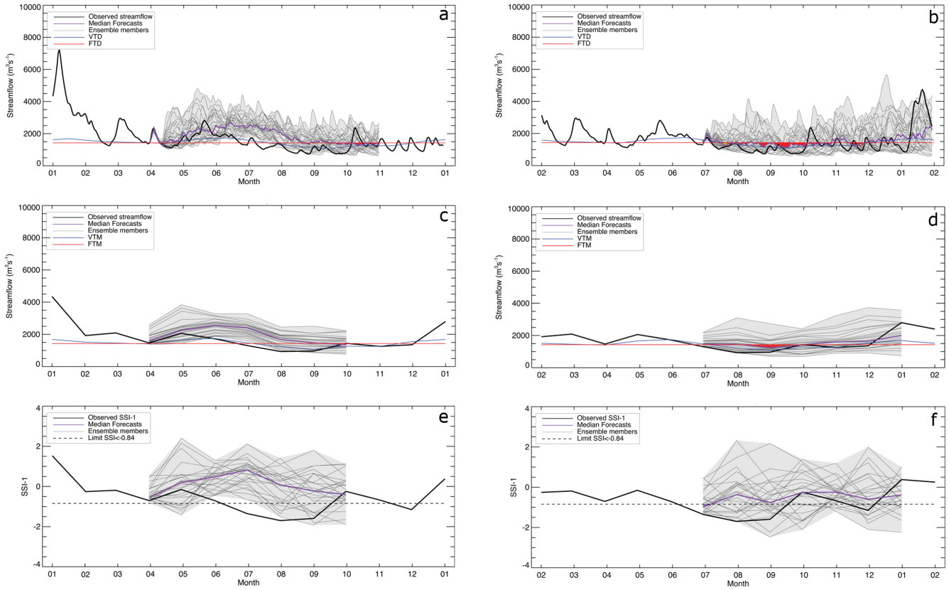
Figure 8. Observed and forecasted streamflow (median and 25 ensemble members) of the Rhine River: a) daily streamflow drought (VTD and FTD) initiated on 1 st April 2003 for 7 months ahead, c) monthly streamflow drought (VTM and FTM) initiated on 1 st April 2003 for 7 months ahead, and e) forecasted SSI-1 drought initiated on 1 st April 2003 for 7 months ahead. b), d), and f) same as a, c, and e, but for forecasts initiated on 1 st July 2003. Droughts are indicated by blue shaded area for VTD and VTM, red shaded area for FTD and FTM, and purple shaded area for SSI-1. Orange areas indicate both VTD and FTD drought.
