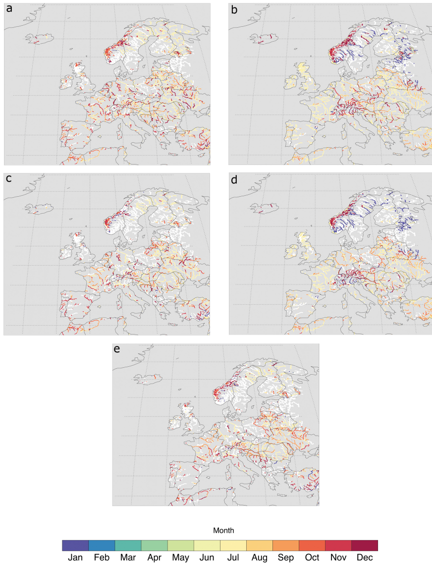
Figure 7. Forecasted drought timing (onset) in the European rivers using different drought identification methods and the forecast initiated on 1 st July 2003 with a lead time 7-month for: a) the VTD drought, b) the FTD drought, c) the VTM drought, d) the FTM drought, and e) the SSI-1 drought. White river color indicates that no drought was forecasted. Please note that in this case drought cannot start in Feb-June.
