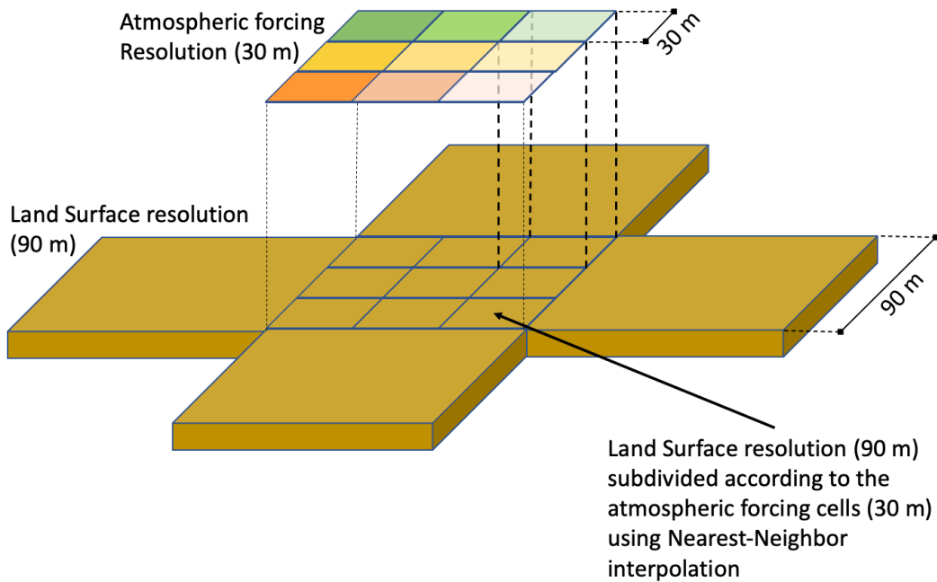
Fig. 1. Example of 30 m atmospheric resolution applied to a 90 m land surface resolution.
