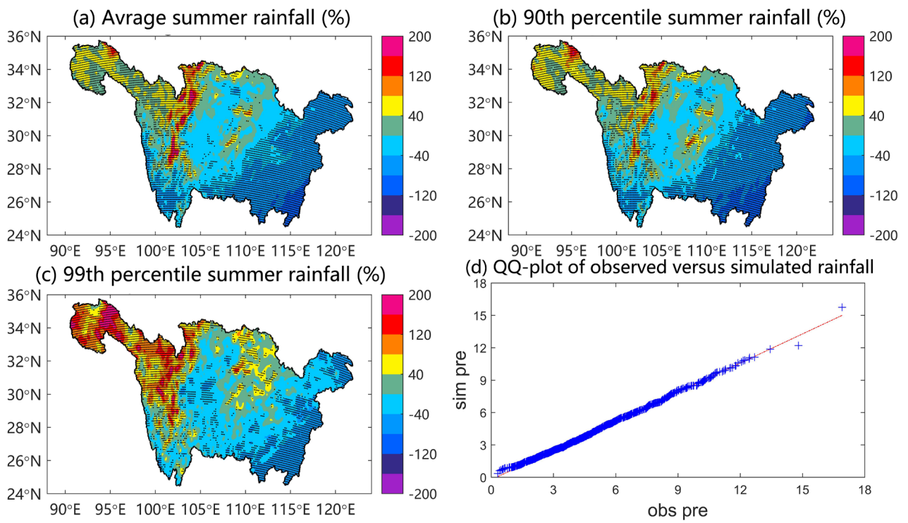
Figure 4. The bias of (a) average summer rainfall (%), (b) 90th percentile summer rainfall (%) and (c) 99th percentile summer rainfall (%) between the 2010 scenario and observed data, and (d) the qq-plot of observed rainfall versus simulated rainfall. The stippling regions show statistically significance of bias identified by t-test at a 5% significance level.
