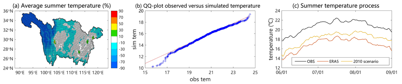
690 Figure 6. (a) The biases of average summer temperature (%) between the 2010 scenario and observed data, the stippling regions show statistically significance of bias identified by t-test at a 5% significance level.; (b) The qq-plot of observed temperature versus simulated temperature; (c) The basin-averaged summer temperature processes of observation, ERA5 and 2010 scenario.
