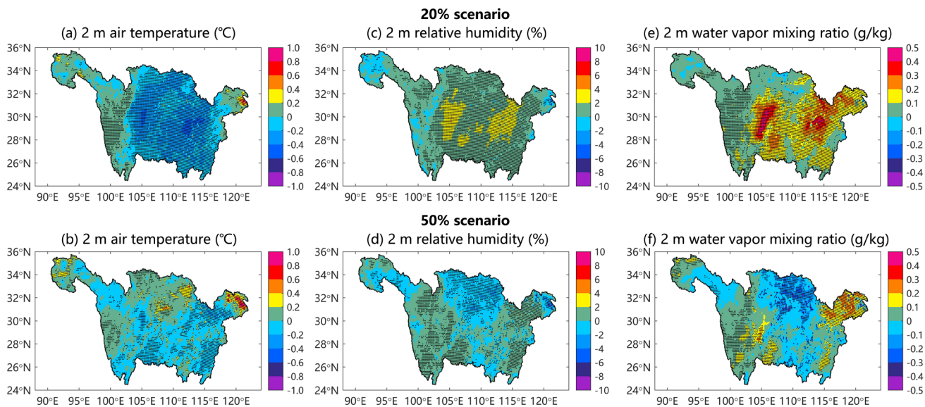
Figure 14. The changes in (a-b) 2m air temperature (°C), (c-d) 2m relative humidity (%) and (e-f) 2m water vapor mixing ratio (g/kg) between the 20% scenario and 2010 scenario, and between the 50% scenario and 2010 scenario. The stippling regions show statistically significance of changes identified by t-test at a 5% significance level.
