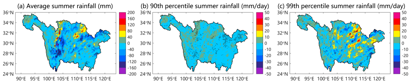
695 Figure 7. The changes in (a) average summer rainfall (mm), (b) 90th percentile summer rainfall (mm/day) and (c) 99th percentile summer rainfall (mm/day) between the 2010 scenario and 1990 scenario. The stippling regions show statistically significance of changes identified by t-test at a 5% significance level.
