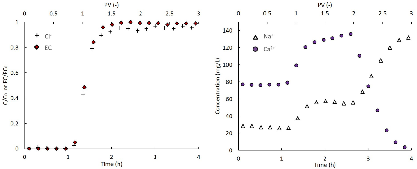
Figure 3. Outflow values versus time (bottom horizontal axis) and pore volume (PV; upper horizontal axis) of (a) measured Cl^- and EC (+ signs and red rhombi), and (b) Na^+ and Ca^{2+} ions (empty triangles and purple circles).
