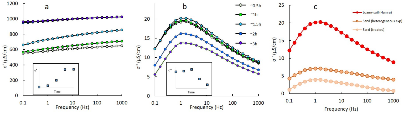
Figure 2. Real (a) and imaginary (b) conductivity between 0.1 and 1000Hz at five different times ( \sim 0.5h, \sim 1h, \sim 1.5h, \sim 2h, \sim 3h ) for the loamy soil. The inserts in (a) and (b) schematically present the dynamics of the real and imaginary conductivity at 1Hz. (c) shows the imaginary conductivity of the three soils used in this work: loamy soil, sand (untreated; used for the heterogeneous experiment) and treated sand.
