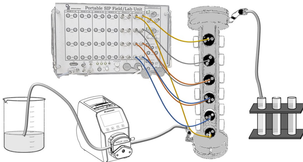
Figure 1. Laboratory setup: the inflow solution is pumped into the column from its bottom and the outflow is collected in fractions. SIP signal is measured between three sets of potential electrodes: channel 1 (blue), channel 2 (orange) and channel 3 (grey). The current is injected between the top and bottom electrodes (yellow).
