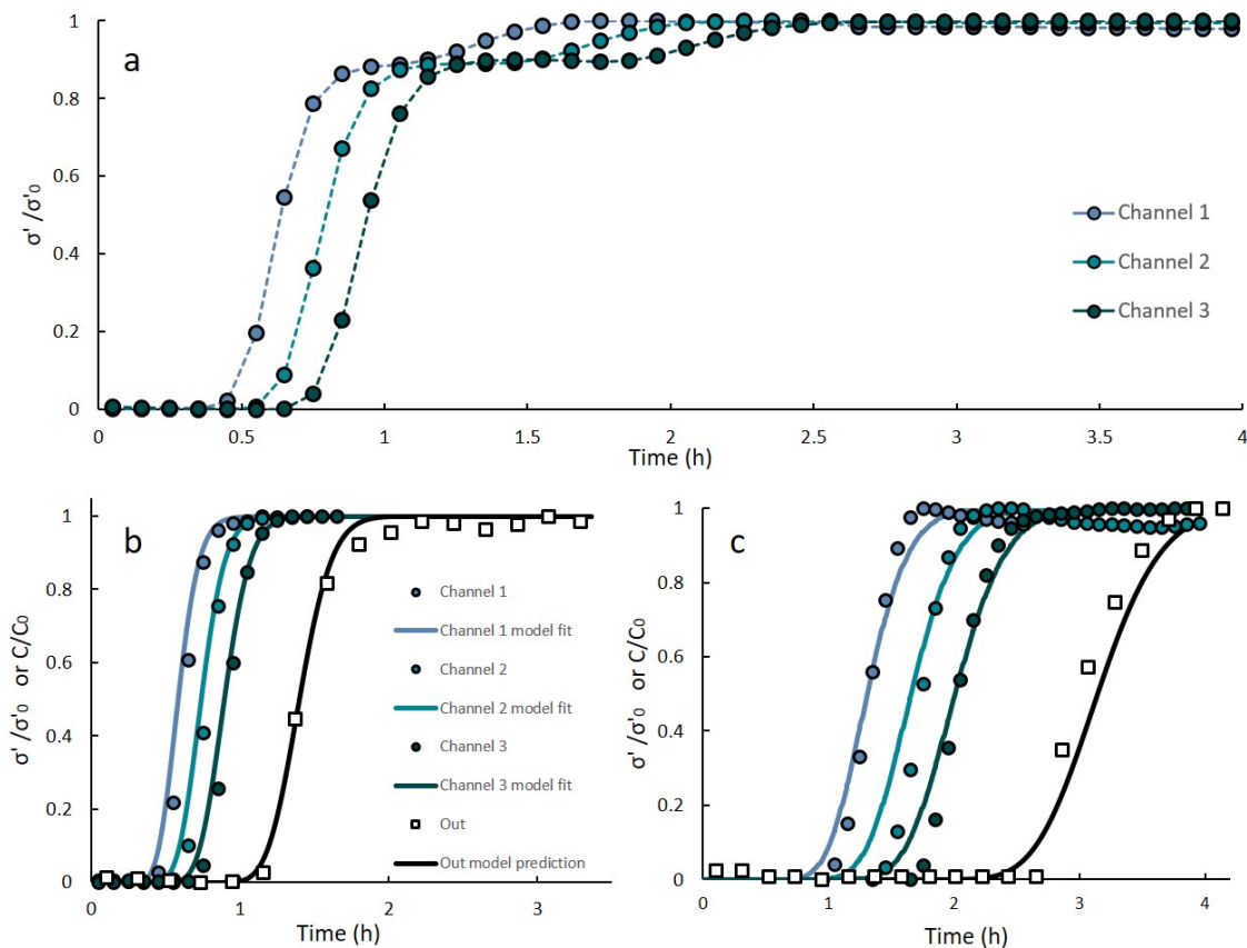
Figure 4. (a) Real conductivity at 1Hz versus time at three locations, (b) model fit to the \sigma' -based initial BT and model prediction for the non-reactive species at the outflow compared to their measured concentration, (c) model fit to the \sigma' -based secondary BT and model prediction for Ca^{2+} at the outflow compared to its measured concentration.
