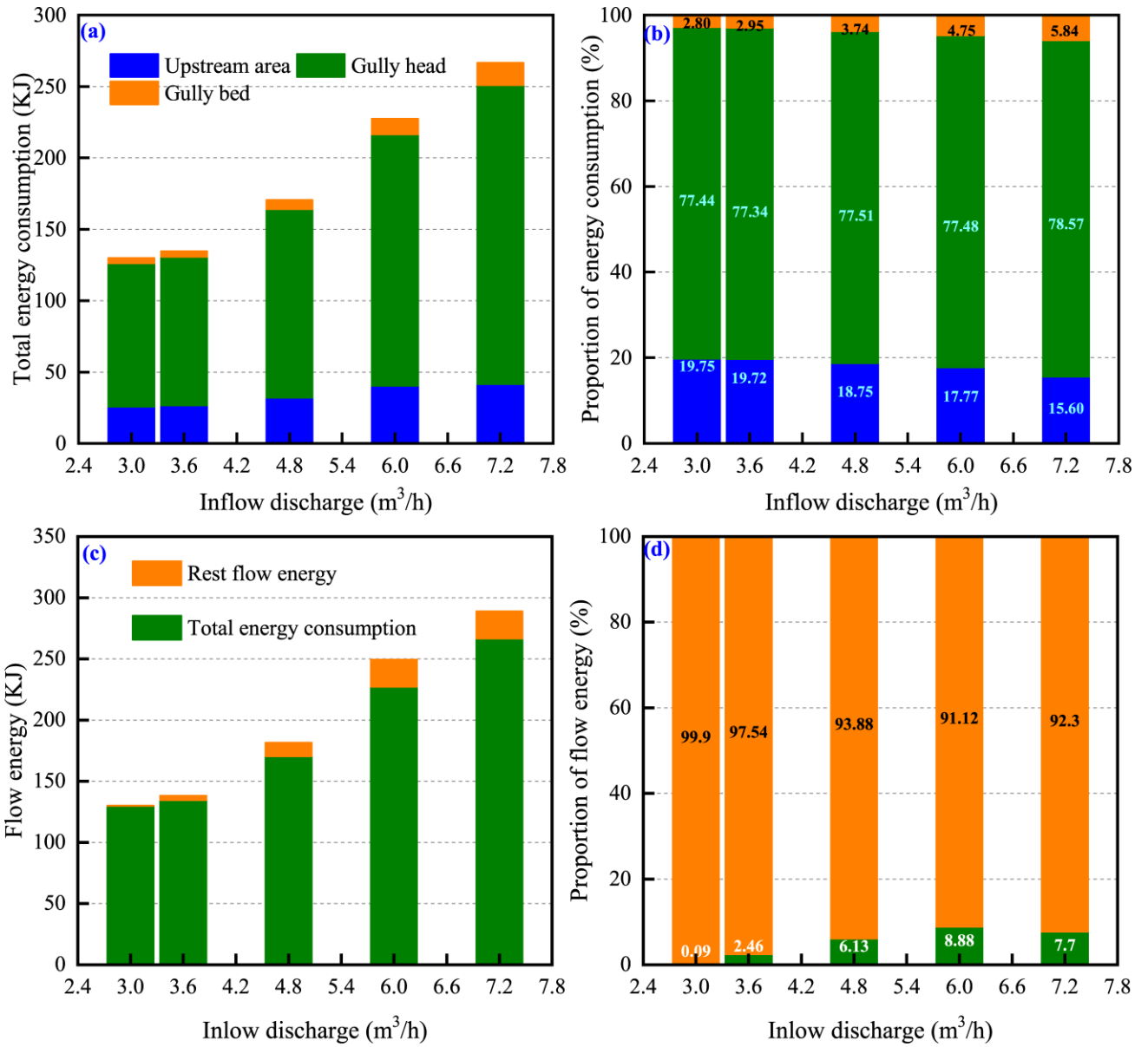
Figure10 Variation in energy consumption of upstream area, gully head and gully bed and their proportions with inflow discharge
