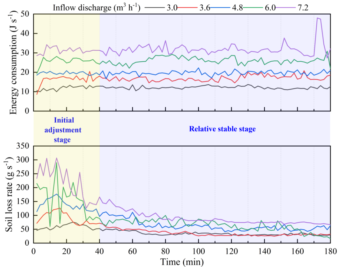
Fig. 3 Relationship between soil loss rate of “UA-GH-GB” system and energy dissipation during headcut erosion
