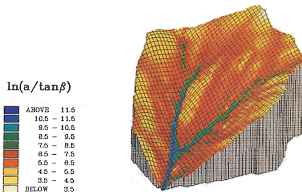
Figure 6. Pattern of topographic index for the Rigelbach catchment, Vosges, France superimposed on a digital terrain model (after Ambroise et al., 1996b). The highest values in the valley bottom and convergent hollows will be predicted as saturating first. A small spring in the catchment on the right-hand hillslope, indicating subsurface convergence, is not reflected in the pattern of the index shown on this map since this is based on the topographic flow pathways alone.
