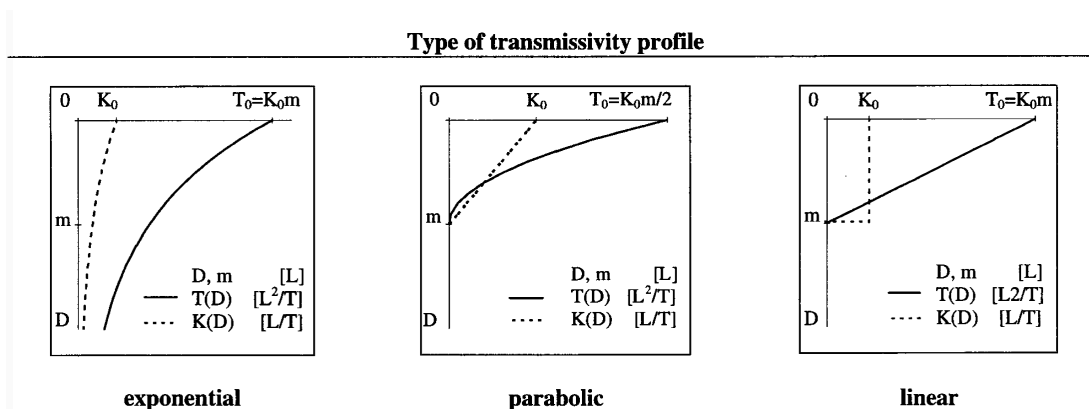
Figure 7. The different types of transmissivity profile considered in Ambroise et al. (1996a).
