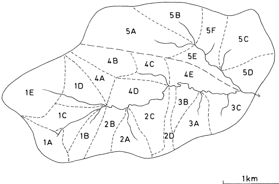
Figure 4. Subdivision of the 8 km 2 Crimble Beck catchment, Yorkshire, UK into 23 headwater and sideslope subcatchments (from Beven and Kirkby, 1979).
