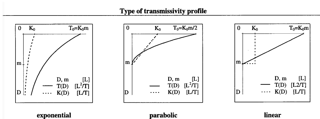
Figure 7. The different types of transmissivity profile considered in Ambroise et al. (1996a). Note that plotting recession discharges against time for the exponential profile 1/Q_b should plot linearly. For the parabolic profile 1/\sqrt{Q_b} should plot linearly (for generalisation to a power law function see Iorgulescu and Musy, 1997; Duan and Miller, 1997), and for the linear profile, \ln Q_b should plot linearly (see Ambroise et al., 1996a).
