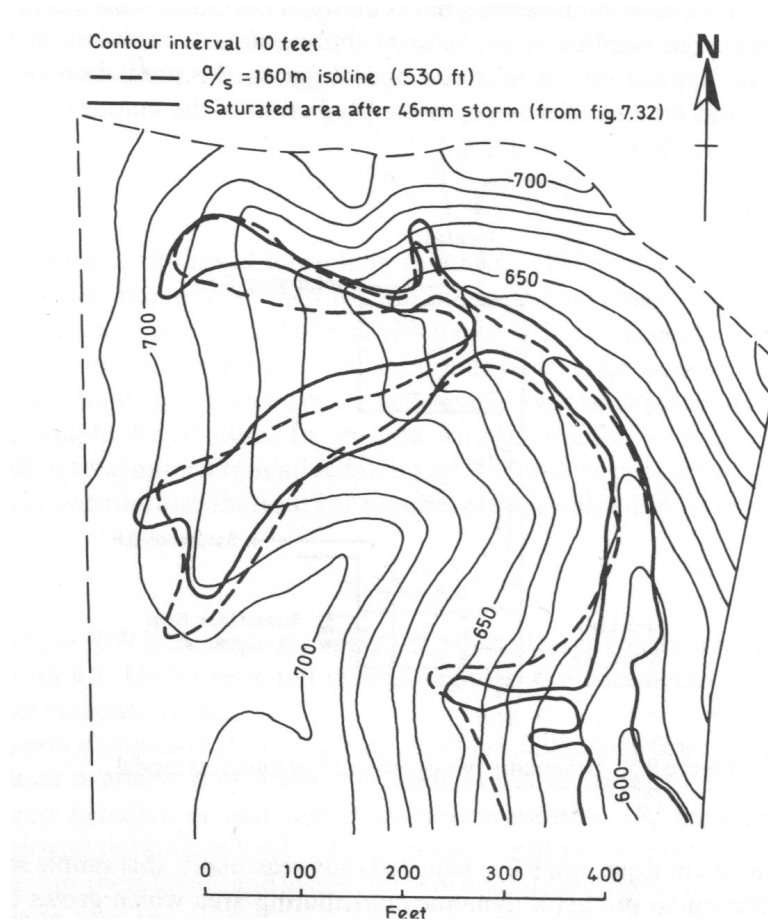
Figure 1. Distribution of the topographic index ( a/\tan \beta ) for the upper East Twin catchment, Mendips, UK (from Kirkby, 1975)
