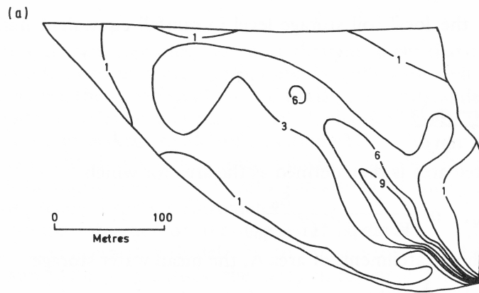
Figure 1. Distribution of the topographic index ( a/\tan \beta ) for the upper East Twin catchment, Mendips, UK (from Kirkby, 1975)
