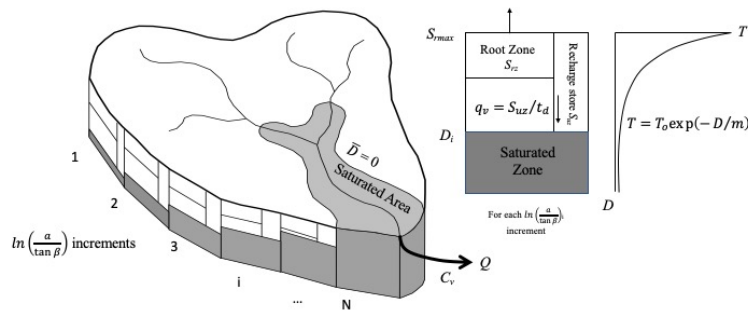
175 Figure 3. Schematic of the classical version of Topmodel (see Table 1 for the definition of the parameters)
