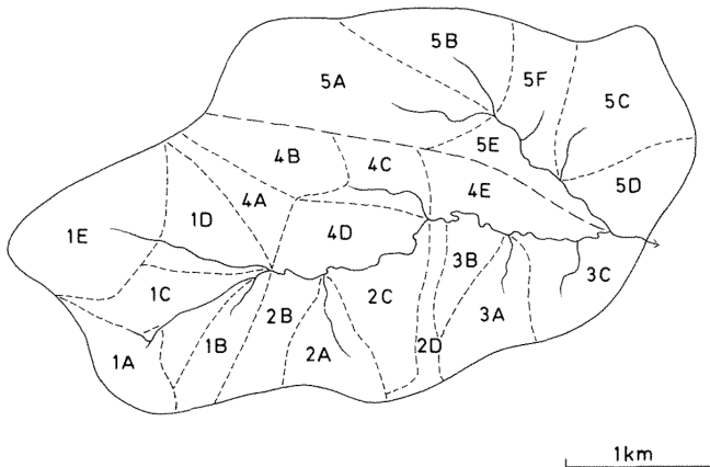
265 Figure 4. Subdivision of the 8 km 2 Crimple Beck catchment, Yorkshire, UK into 23 headwater and sideslope subcatchments (from Beven and Kirkby, 1979).
