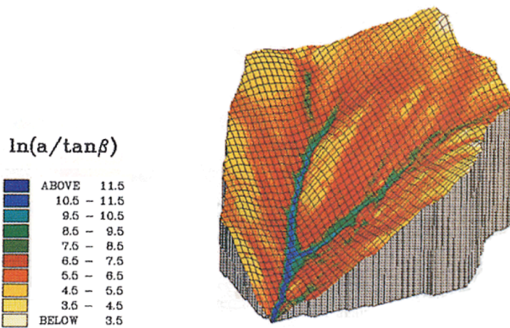
Figure 6. Pattern of topographic index for the Rinkelbach catchment, Vosges, France superimposed on a digital terrain model (after Ambroise et al., 1996b). The highest values in the valley bottom and convergent hollows will be predicted as saturating first. A small spring in the catchment on the right-hand hillslope, indicating subsurface convergence, is not reflected in the pattern of the index shown on this map since this is based on the topographic flow pathways alone.
