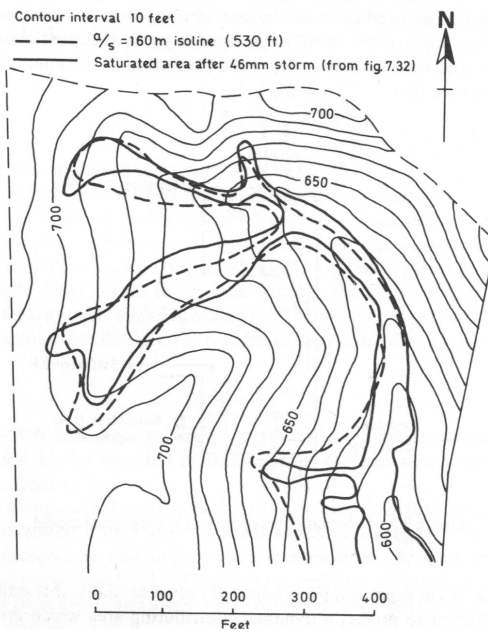
Figure 1. Distribution of the topographic index ( a/\tan\beta ) for the upper East Twin catchment, Mendips, UK (from Kirkby, 1975)
