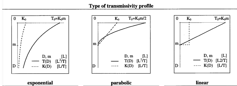
545 Figure 7. The different types of transmissivity profile considered in Ambroise et al. (1996a). Note that plotting recession discharges against time for the exponential profile 1/Q_b should plot linearly. For the parabolic profile 1/\sqrt{Q_b} should plot linearly (for generalisation to a power law function see Iorgulescu and Musy, 1997; Duan and Miller, 1997), and for the linear profile, \ln Q_b should plot linearly (see Ambroise et al., 1996a).
