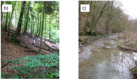
Figure 1. a) map of the Colpach catchment (location northern Luxembourg), b) picture of a typical forested hillslope within the Colpach catchment, c) the Colpach river around 4 km north of the gauging station.
