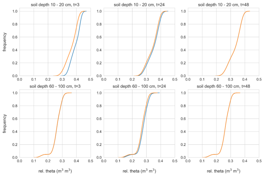
Figure 8. Relative soil moisture distributions for two gridded hillslope models that received the lowest (orange curve) respectively the highest (blue curve) amount of rainfall during event I ( 15 \text{ mm } 5 \text{ hr}^{-1} and 30 \text{ mm } 5 \text{ hr}^{-1} ). Presented for time step t = 3 (during the event), t = 24 (after the event), and t = 48 (after the event).
