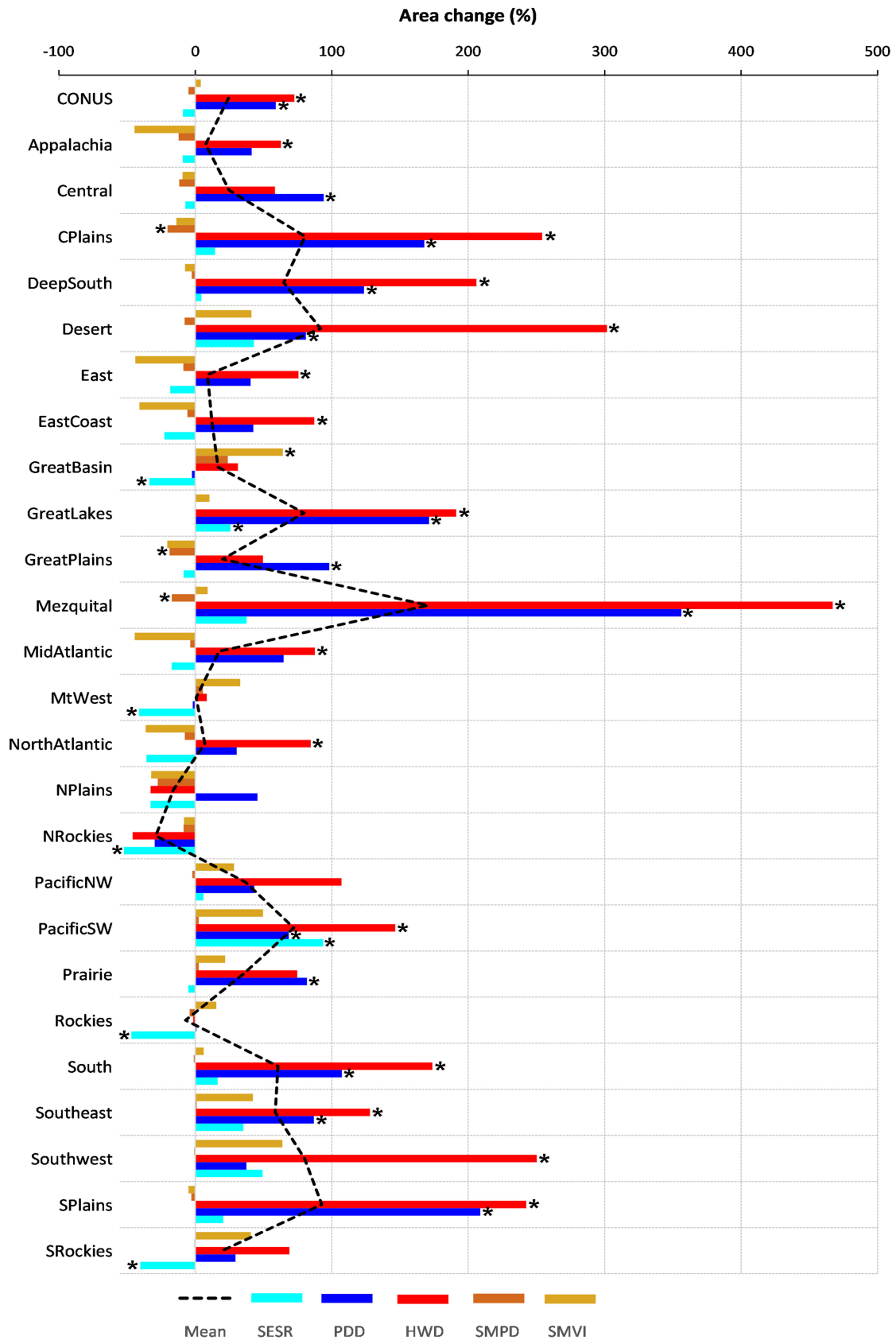
429 Figure 8: Percentage change in areas hit by flash drought in (2009-2018) compared to (1979-1989) for CONUS and all Bukovsky 430 regions. Dashed black line represents the mean of all definitions per region. Significant trends (according to the Mann-Kendall 431 test) are marked by asterisks.
