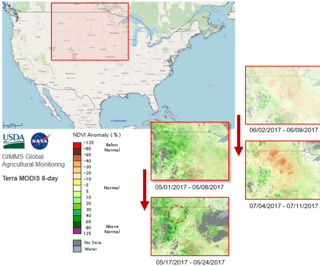
Fig. 2. Similar to Fig. S2 for 2017 flash drought.
