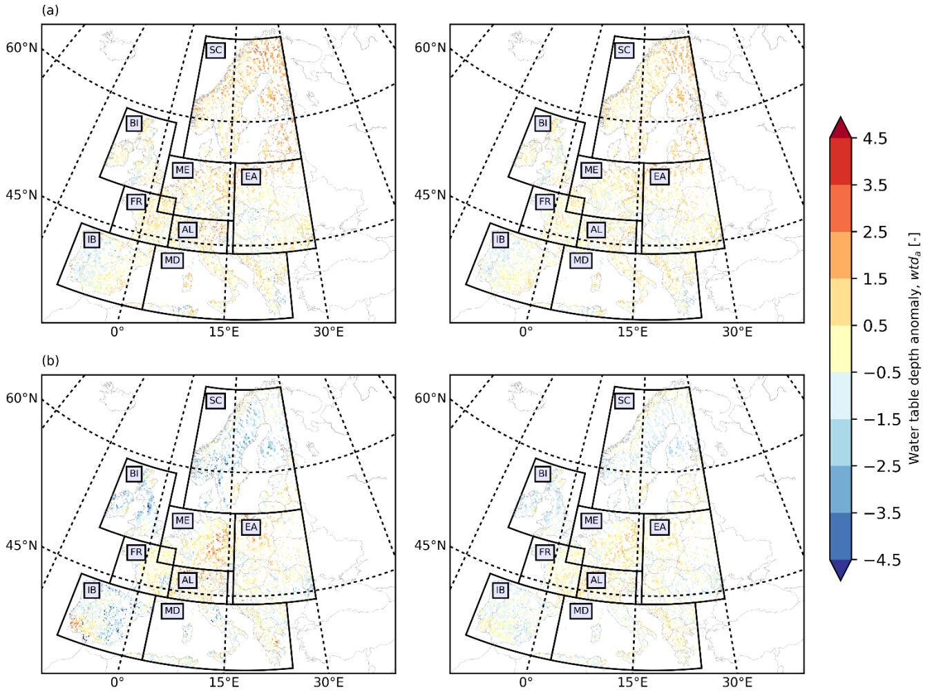
315 Figure 5: European wtd_a maps for (a) August 2003 (i.e., in the training period); (b) August 2015 (i.e., in the testing period), derived from the TSMP-G2A data set (left) and results from LSTM networks (right).
