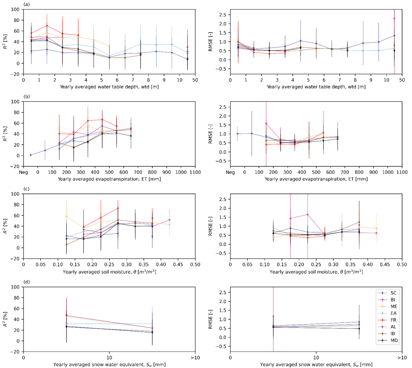
325 Figure 6: Averages and standard deviations of the test R^2 scores (left) and RMSEs (right) over the categorized results: yearly averaged (a) wtd ; (b) ET ; (c) \theta ; (d) S_w . The averages are indicated as dots, while the bars indicate standard deviations. The different colors reflect test results in different PRUDENCE regions.
