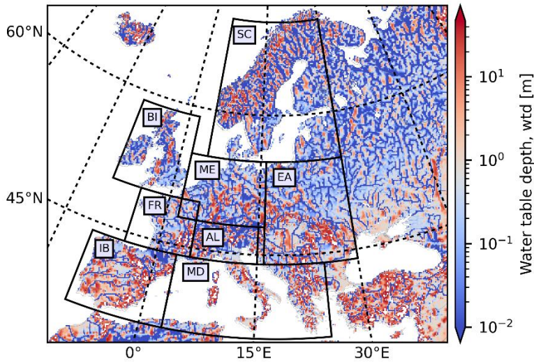
215 Figure 3: TSMP-G2A wtd [m] climatology over the European continent for the time period 1996 to 2016. Areas bounded by the thick black lines show the PRUDENCE regions (i.e., SC: Scandinavia; BI: British Isles; ME: Mid-Europe; EA: Eastern Europe; FR: France; AL: Alps; IB: Iberian Peninsula; MD: Mediterranean).
