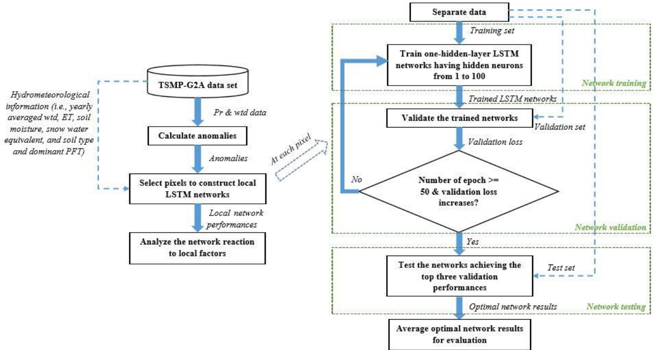
290 Figure 4: Workflow for LSTM network setup over the European CORDEX domain. The left section represents the overall processes of the network setup, whereas the right section shows how to apply LSTM networks at a selected pixel. The blue dashed lines with arrows indicate additional data transmission paths.
