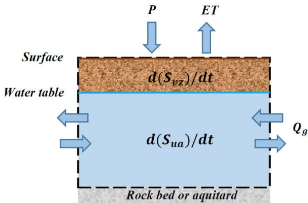
Figure 1: Conceptual model of groundwater balance over a control volume (after Maxwell, 2010). P is precipitation; ET is actual evapotranspiration; Q_g is the lateral groundwater flow; S_{vz} and S_{ua} are the water storages in the vadose zone and the unconfined aquifer, respectively; and t is time.
