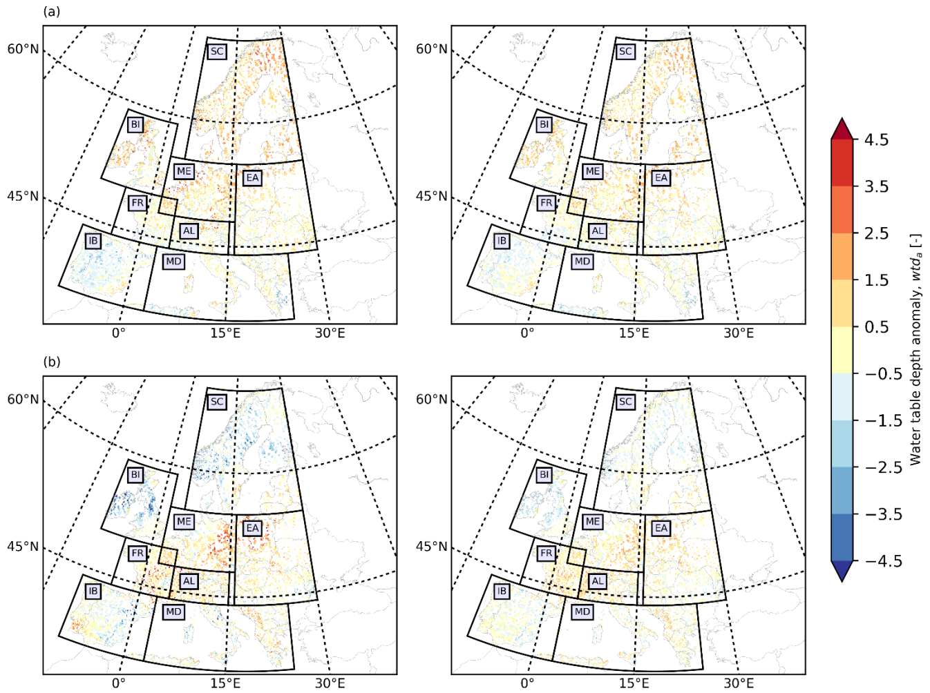
Figure B2: European wtd_a maps for (a) December 2003; (i.e., in the training period); (b) December 2015; (i.e., in the testing period), derived from the TSMP-G2A data set (left) and results from LSTM networks (right).
