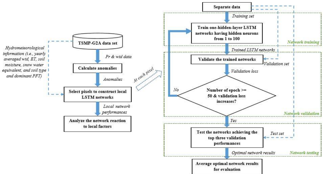
310 Figure 4: Workflow for LSTM network setup over the European CORDEX domain. The left section represents the overall processes of the network setup, whereas the right section shows how to apply LSTM networks at a selected pixel. The dash blue dashed lines with arrows indicate additional data transmission paths.
