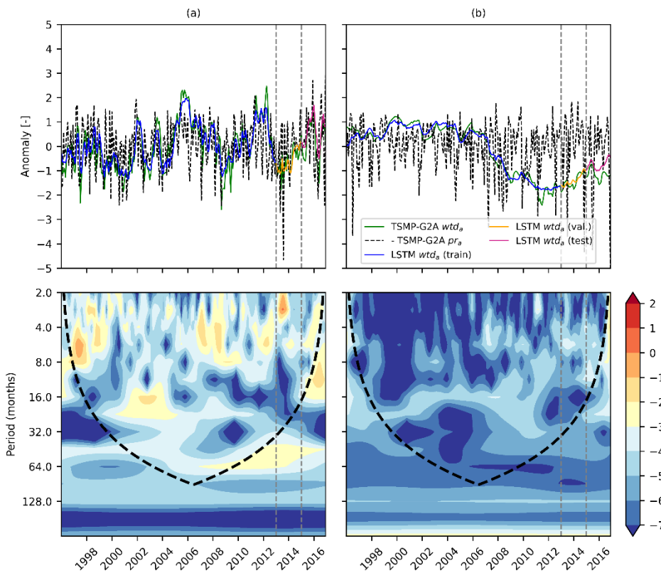
555 Figure C1: -TSMP-G2A pr_a , TSMP-G2A wtd_a and LSTM wtd_a time series (top) as well as cross-wavelet spectra for TSMP-G2A pr_a and wtd_a series (bottom) at (a) Pixel 43; (b) Pixel 5; (c) Pixel 64. The lines have the same definitions as Fig. 9.
