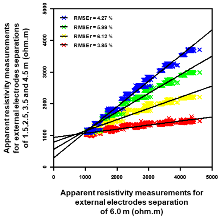
Figure 6: Scatter plots showing the first apparent resistivity level for an ES of 2 m (external electrodes spacing of 6 m) versus the four surficial apparent resistivity levels for an ES of 0.5 m with external electrodes separations of 1.5 (red crosses), 2.5 (yellow crosses), 3.5 (green crosses) and 4.5 m (blue crosses) using the Wenner-Schlumberger array for the 25 synthetic resistivity models. The linear regressions correspond to the thick black lines and their accuracy is indicated by the root mean square relative error (RMSEr).
