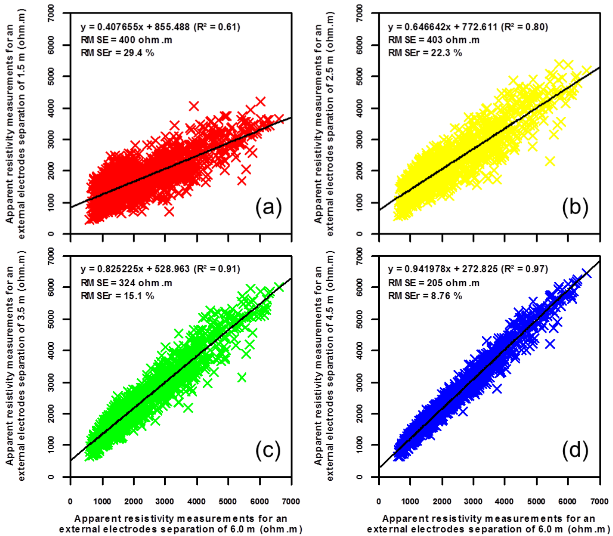
Figure 10: Scatter plots showing the first apparent resistivity level for an ES of 2 m (external electrodes spacing of 6 m) versus the first four surficial apparent resistivity levels for an ES of 0.5 m with external electrodes separations of 1.5 (red crosses), 2.5 (yellow crosses), 3.5 (green crosses) and 4.5 m (blue crosses) for the 12 plot scale ERT profiles measured in the Weierbach catchment. The linear regressions correspond to the thick black lines and their accuracy is indicated by the coefficient of determination ( R^2 ), the root mean square error (RMSE) and the root mean square relative error (RMSEr).
