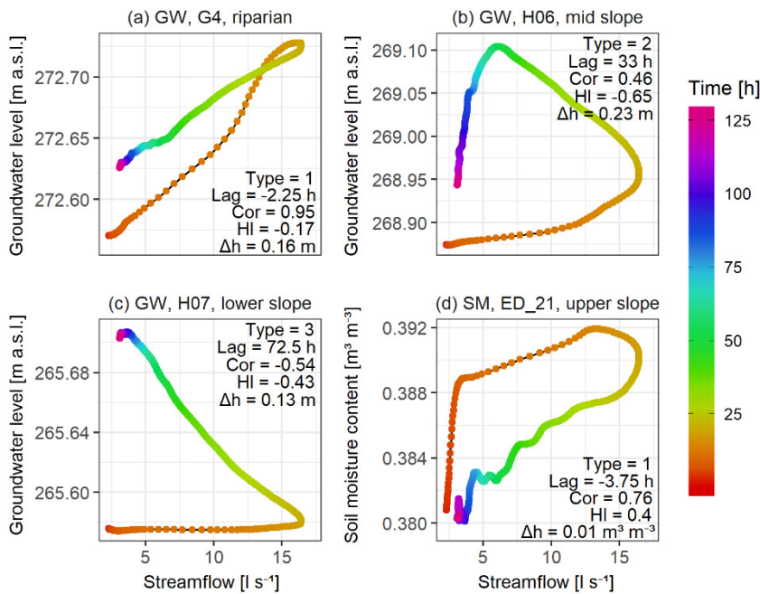
3.2.2 Figure 10: Hysteresis loops for the event 29 (2017-12-21) (Fig. 3, left column). Each panel represents different response type: (a) type 1 groundwater (GW) response; (b) type 2 GW response, (c) type 3 GW response; (d) type 1 soil moisture (SM) response. Colour of points represents the time since the start of the event. Event dynamics of each station in relation to the streamflow is described by the response type (Type), peak-to-peak time (Lag), Spearman correlation coefficient (Cor), hysteresis index (HI) and groundwater table or soil moisture content change over the event ( \Delta h ). Spatial patterns of event response types
