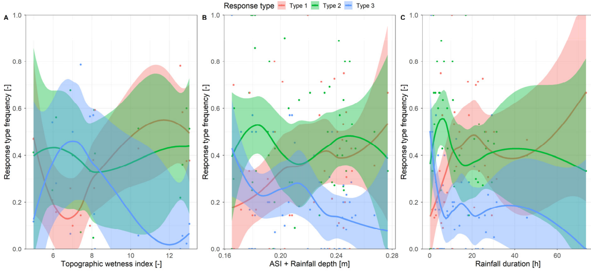
640 Figure A2: Groundwater response type frequency over stations topographic wetness index (a), a sum of antecedent wetness (ASI) and event rainfall depth (b) and rainfall event duration (c). Colours represent different response types as defined in section 2.6. Points are calculated values of response type frequencies; lines are local regression fits for each response type and the shaded areas corresponding 95% confidence intervals.
