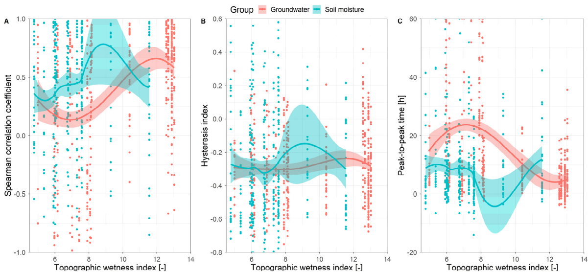
635 Figure A1: Spearman correlation coefficient (a), hysteresis index (b) and peak-to-peak time (c) of groundwater and soil moisture responses to streamflow event responses over locations with different topographic wetness indices. Colours represent different variable group, i.e. groundwater and soil moisture. Points are calculated values for a single event and station; lines are local regression fits for each variable group and shaded areas the corresponding 95% confidence intervals.
