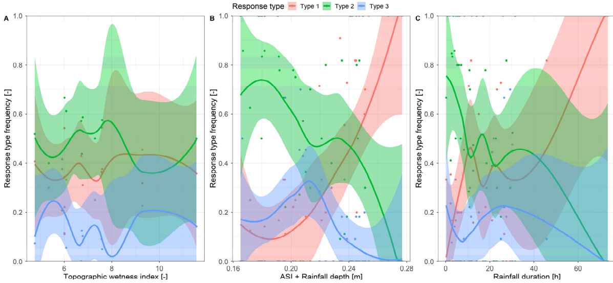
645 Figure A3: Soil moisture response type frequency over stations topographic wetness index (a), a sum of antecedent wetness (ASI) and event rainfall depth (b) and rainfall event duration (c). Colours represent different response types as defined in section 2.6. Points are calculated values of response type frequencies; lines are local regression fits for each response type and the shaded areas corresponding 95% confidence intervals.
