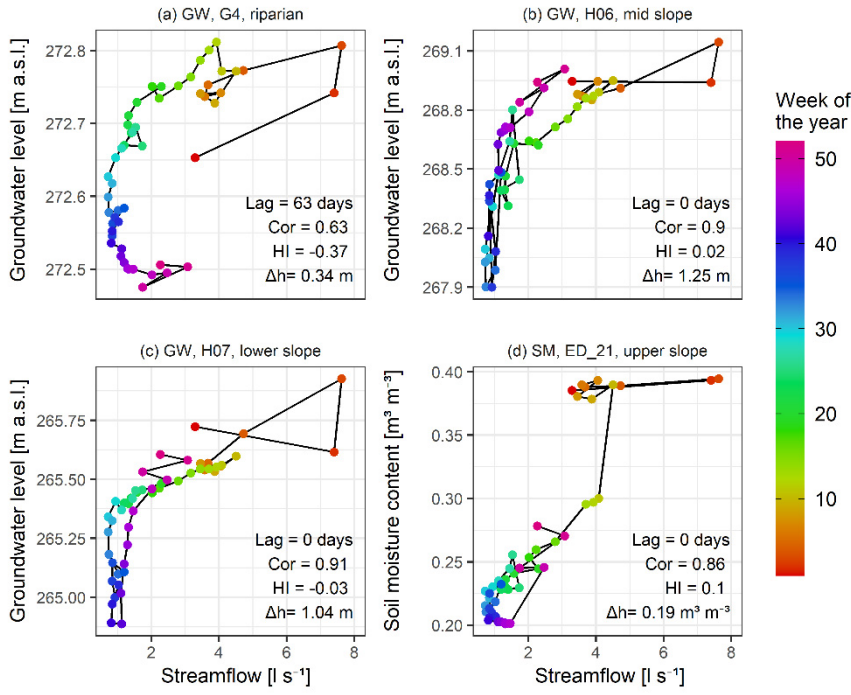
Figure 12: Seasonal hysteresis loops of three groundwater stations (a, b, c) and one soil moisture station (d) to the streamflow for the year 2018 (Fig. 4). Colour of the points represents the week of the year. Seasonal dynamics of each station in relation to the streamflow is described by time shift in seasonal dynamics (Lag), Spearman correlation (Cor), hysteresis index (HI) and groundwater table elevation or soil moisture content change over the year ( \Delta h ).
