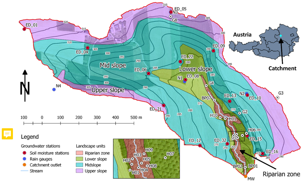
Figure 1: Hydrological Open Air Laboratory in Petzenkirchen, Lower Austria. Coloured areas represent different landscape units defined based on the Topographic Position Index, which compares the elevation of a point and the mean elevation of its surrounding. Elevation contours lines with a 5 m interval are given in black. The inset map is the detail of the area marked by a black rectangle on the main map.
