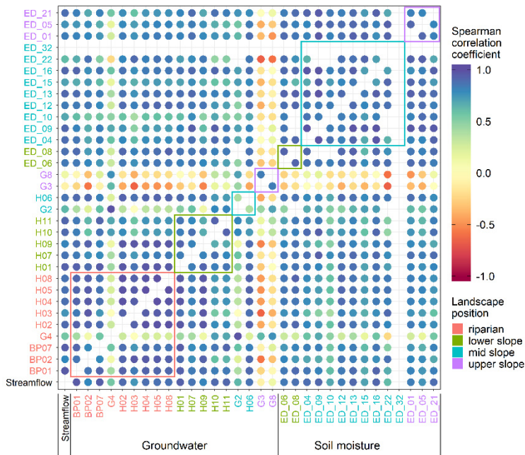
Figure 13: Median Spearman correlation coefficient between median weekly streamflow at catchment outlet (Q), groundwater (BP**, H**, G*) and soil moisture (ED_**) over years 2017 and 2018. Colour of the circles corresponds to the value of the Spearman correlation coefficient; Colour of the station names corresponds to their landscape unit. Coloured rectangles enclose values of stations in the same landscape unit. Only time-series longer than 45 weeks per year are compared.
