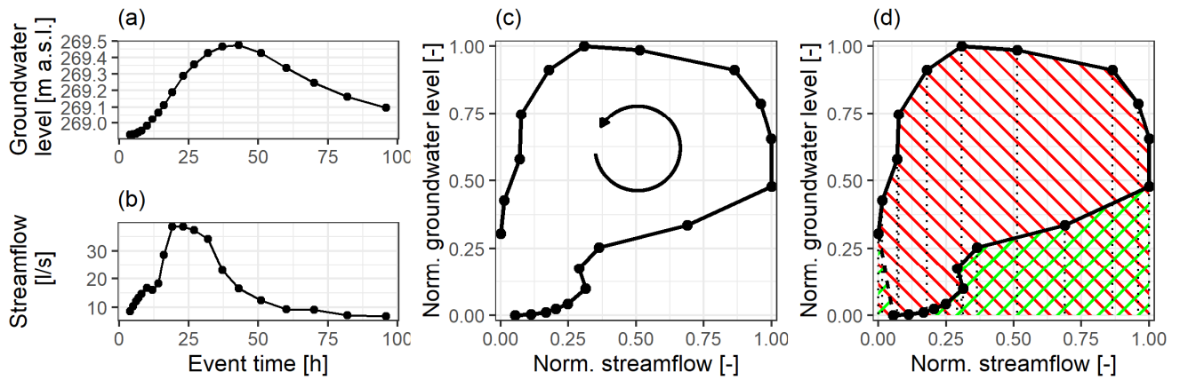
675 Figure B1: Example of the hysteresis index calculation: (a) and (b) show original groundwater and streamflow time-series, respectively; (c) shows the counterclockwise hysteresis loop of the normalized time-series from (a) and (b); (d) shows the positive and negative area contributions to the hysteresis index in green and red pattern, respectively. Hysteresis index is -0.64.
