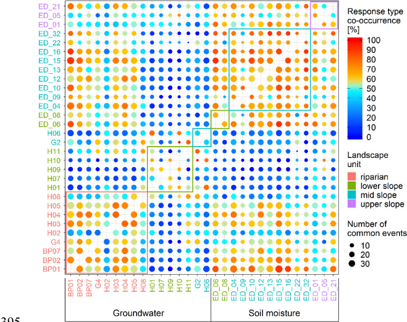
Figure 11: The frequency of events when two stations have the response of the same type – i.e. response type co-occurrence. The size of circles corresponds to the number of events when both stations had a response. Colour of the circles corresponds to the frequency of the response type co-occurrence. Colour of the station names corresponds to their landscape unit. Coloured rectangles enclose values of groundwater and soil moisture stations in the same landscape unit.
