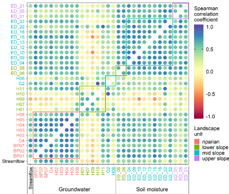
Figure 6: Median Spearman correlation coefficient between streamflow at catchment outlet (Streamflow), groundwater stations (BP**, H**, G*) and soil moisture stations (ED_**) for all events. Colour of the circles corresponds to the Spearman correlation coefficient; Colour of the station names corresponds to their landscape unit. Coloured rectangles enclose correlations of stations in the same landscape unit.
