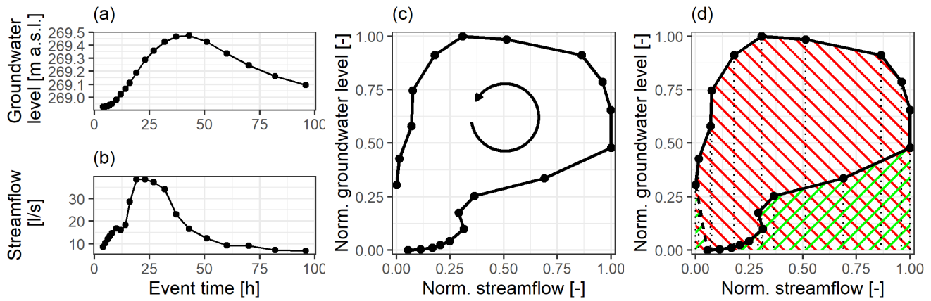
Figure B1: Example of the hysteresis index calculation: (a) and (b) show original groundwater and streamflow time-series, respectively; (c) shows the counter-clockwise hysteresis loop of the normalized time-series from (a) and (b); (d) shows the positive and negative area contributions to the hysteresis index in a green and red pattern, respectively. Hysteresis index is -0.64.
