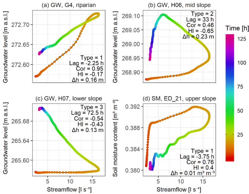
Figure 10: Hysteresis loops for the event 29 (2017-12-21) (Fig. 3c, left column). Each panel represents a different response type: (a) type 1 groundwater (GW) response; (b) type 2 GW response, (c) type 3 GW response; (d) type 1 soil moisture (SM) response. The points' Colour of points represents the time since the start of the event. Event dynamics of each station in relation to the streamflow is described by the response type (Type), peak-to-peak time (Lag), Spearman correlation coefficient (Cor), hysteresis index (HI) and groundwater table or soil moisture content change over the event ( \Delta h ).
