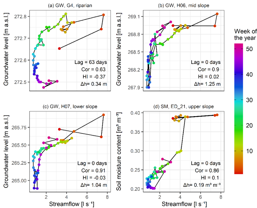
Figure 12: Seasonal hysteresis loops of three groundwater stations (a, b, c) and one soil moisture station (d) to the streamflow for the year 2018 (Fig. 4). Circles' colour represents the week of the year. Seasonal dynamics of each station in 455 relation to the streamflow is described by time-shift in seasonal dynamics (Lag), Spearman correlation (Cor), hysteresis index (HI) and groundwater table elevation or soil moisture content change over the year ( \Delta h ).
