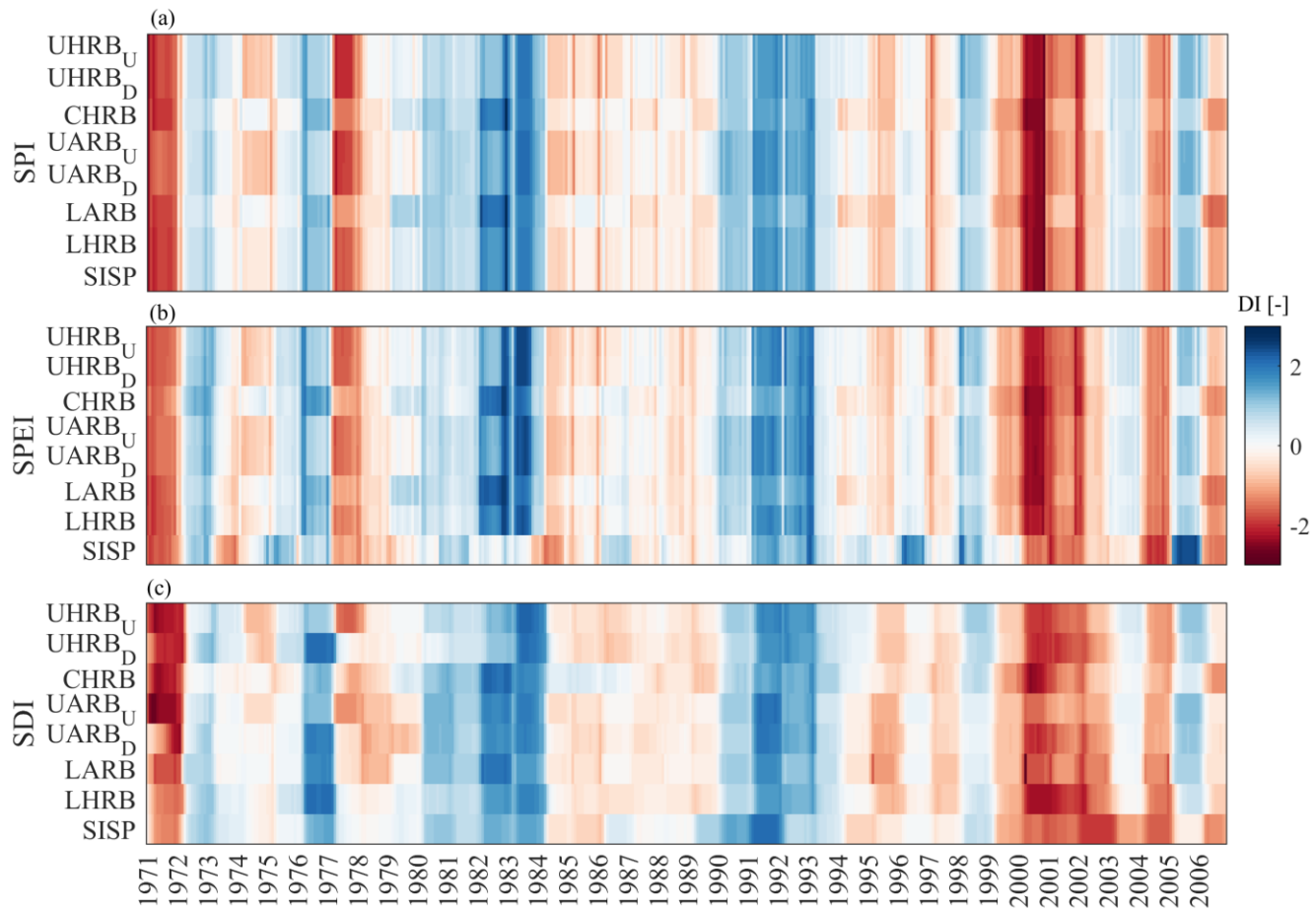
1020 Figure 6. Time series of monthly drought indices (based on 12 months accumulation time) SPI, SPEI and SDI for the sub- basins ID1 – ID8 for the 1970 – 2006 study period
