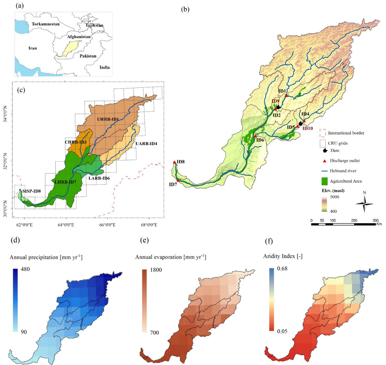
960 Figure 1. (a) The location of Helmand River Basin (HRB) in central Afghanistan, (b) elevation map of the HRB, also indicating the sub-basin boundaries, the locations of the sub-basin outlets and the agriculturally used area (as of 2006), (c) outline of the sub-basins analysed in this study, including the grid cells of CRU precipitation data used, (d) long-term mean annual precipitation P [ \text{mm yr}^{-1} ], (e) long-term mean annual potential evaporation E_P [ \text{mm yr}^{-1} ] and (f) the aridity index I_A = P/E_P [-]
