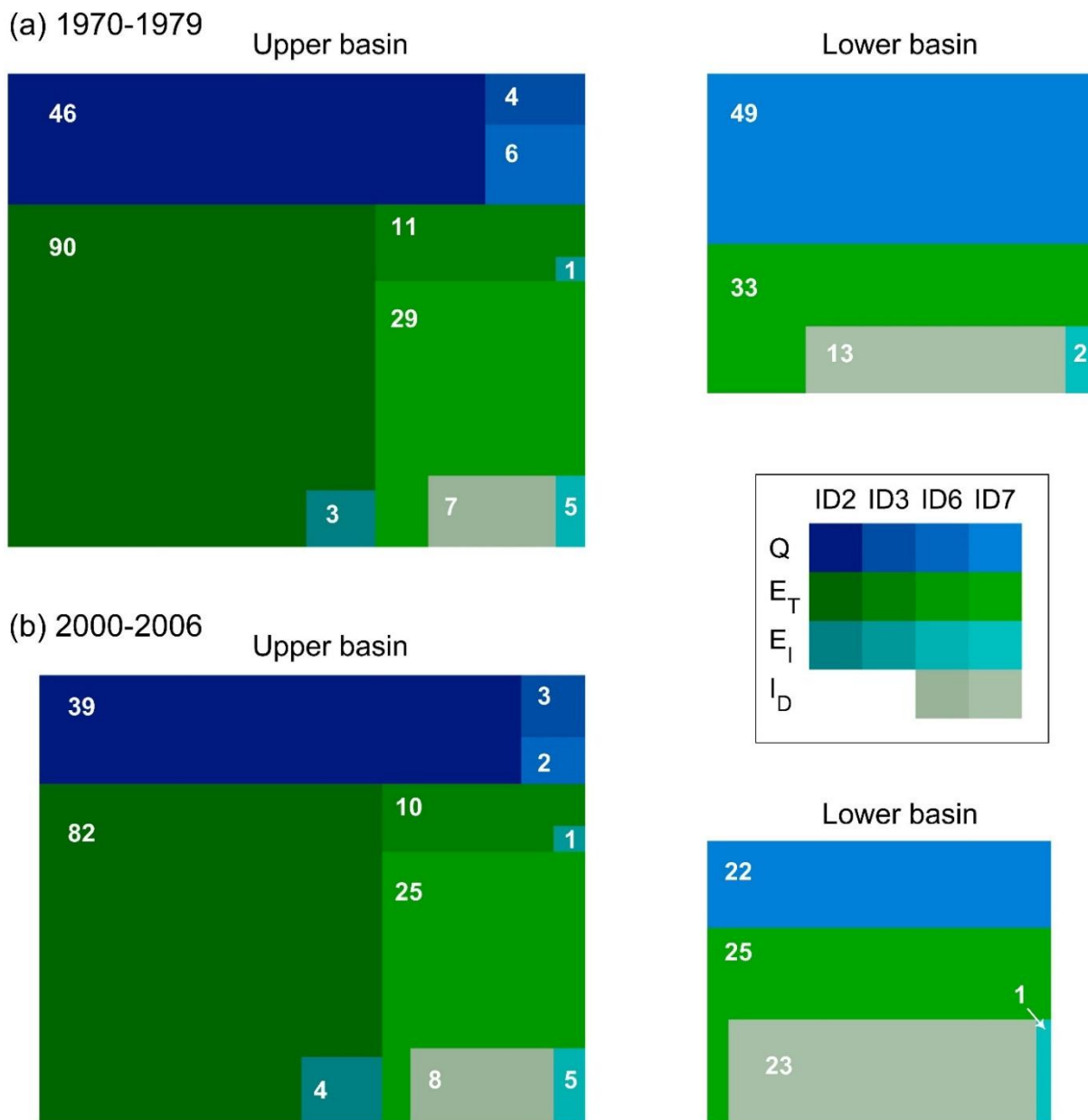
1150 Figure 11. Water balances of the Upper and the Lower basins, respectively for (a) the 1970-79 and (b) the 2000-2006 periods. The size of the outer squares is equivalent to the total water available, i.e. for the upper basin precipitation P , for the lower basin precipitation P plus the combined inflow Q from the upper basin. The size of the internal rectangles of each flux ( Q : streamflow, E_T : transpiration, E_I : interception evaporation and I_D : irrigation demand) in each sub-basin is equivalent to its fraction of the total available water in the upper and lower basin, respectively. The fluxes represent the decadal mean values and are shown in [\text{mm y}^{-1}] .
