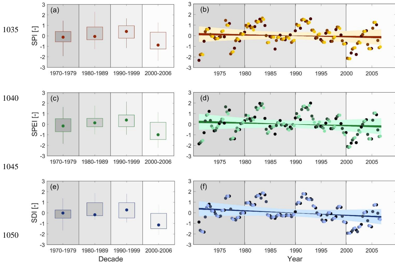
Figure 7. Decadal distributions and time series of mean basin (a)-(b) SPI, (c)-(d) SPEI and (e)-(f) SDI over the study period. The dots in the box plots indicate the median values and the whiskers the 5/95 th percentiles. The dark to light shaded dots in the time series plots indicate the monthly drought indices (based on 12 months accumulation time) for all months of January, April, July and October, respectively. The dark shaded areas indicate the envelope of trend lines for the trends estimated based on all months of January, April, July and October, respectively. The light shaded areas show the associated envelope of 5/95 th confidence intervals.
