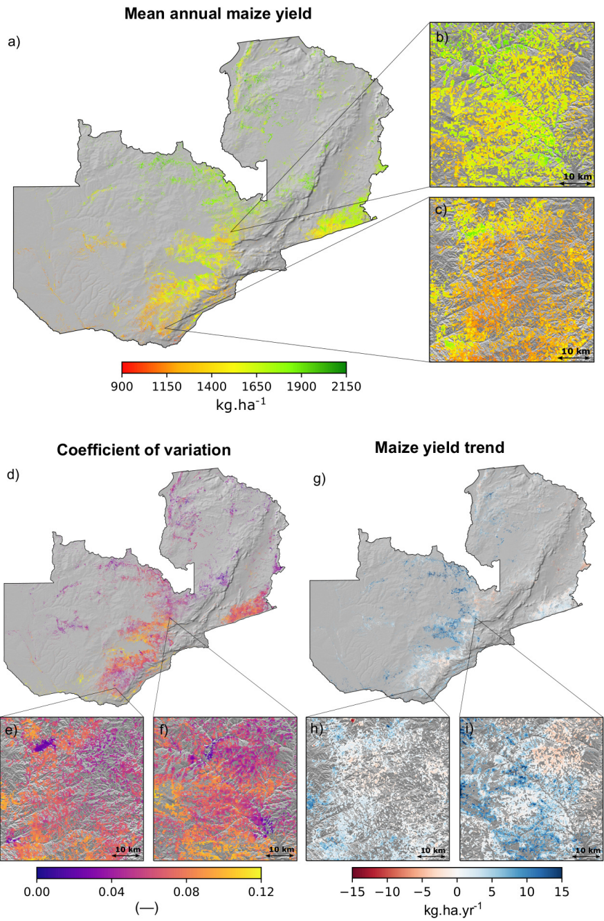
Figure 4. Annual maize yields (a), coefficient of variation (d), and maize yield trends (g) for the period between 2000–2018 estimated using a random forest model. Each zoom panel (b, c, e, f, h, i) shows the respective estimates at a 250-m resolution for a 50-km x 50-km area.
