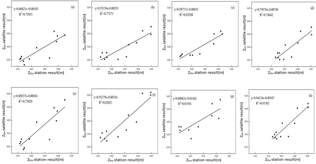
Fig. 7 Scatter plots of the retrieved and calculated surface roughness lengths at four sites
