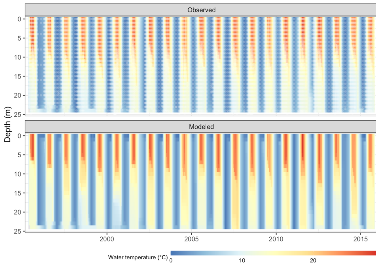
900 Figure 4 Comparison of Lake Mendota water temperature from observations (upper panel, white dots mark sampling events) and GLM-AED2 simulations (lower panel).
