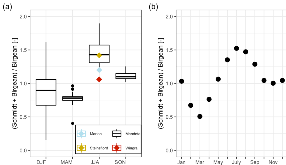
Figure 7 Dynamics of average HBR = (St+B)/B over time. A: Box-plots of HBR over the meteorological seasons, which represent seasonal quarters of the year, beginning in December. The summer HBR values for Lake Marion, Lake Steinsfjord, and Lake Wingra were taken from Kjensmo (1994). B: Scatterplot of average HBR values for each month
