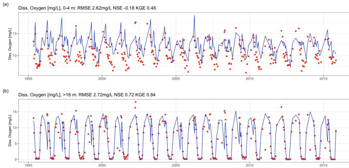
Figure 9 Time-series comparison between observed (red dots) and modeled dissolved oxygen concentrations (blue lines). The fit criteria root-mean square error (RMSE), Nash-Sutcliffe coefficient of efficiency (NSE) and Kling-Gupta coefficient of efficiency (KGE). A: averaged dissolved oxygen concentrations in the epilimnion (0-4 m). B: averaged dissolved oxygen concentrations in the hypolimnion (deeper than 16 m).
