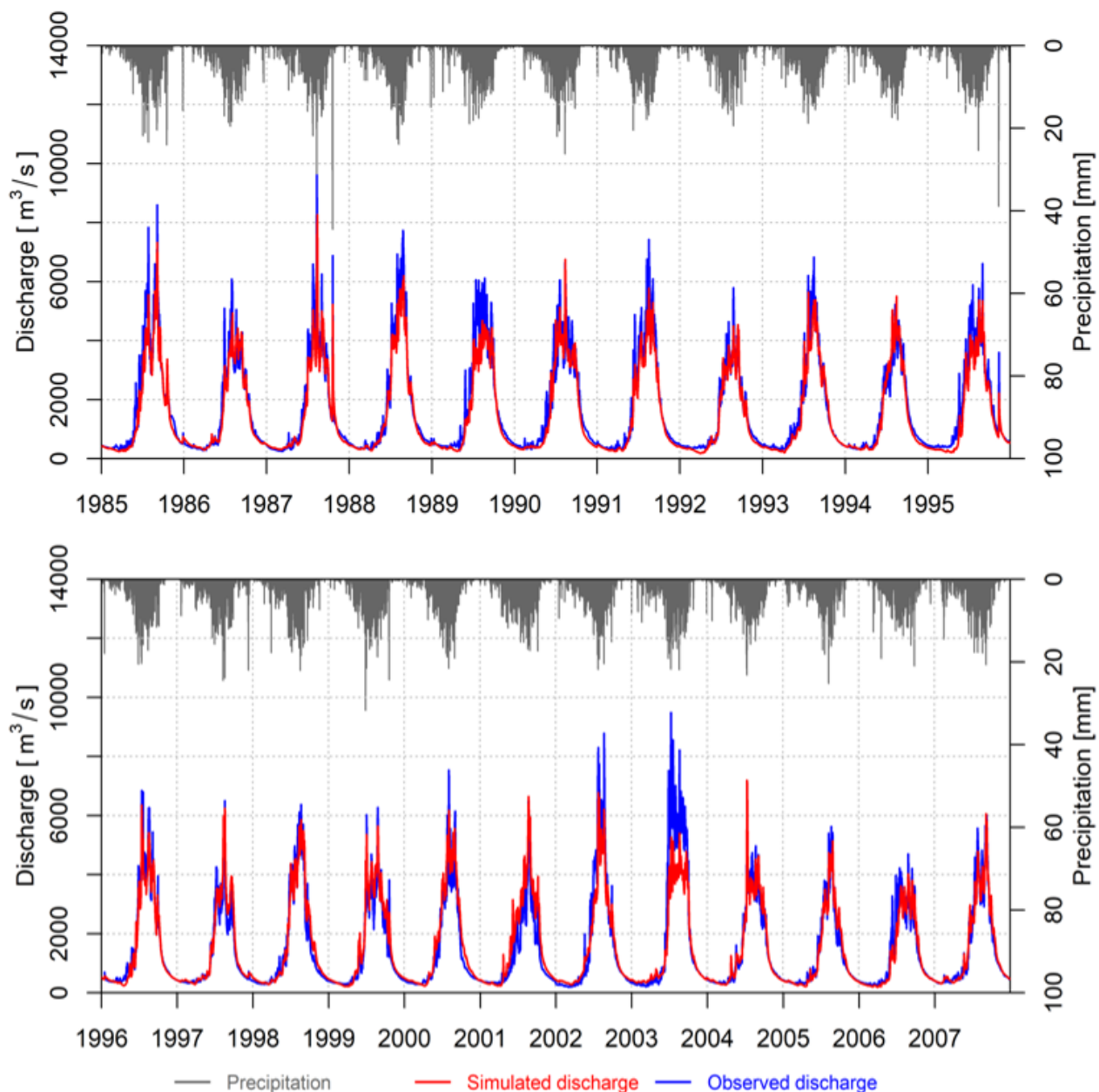
870 Figure 4: Calibration (top) and validation (bottom) of daily streamflow at Chatara
