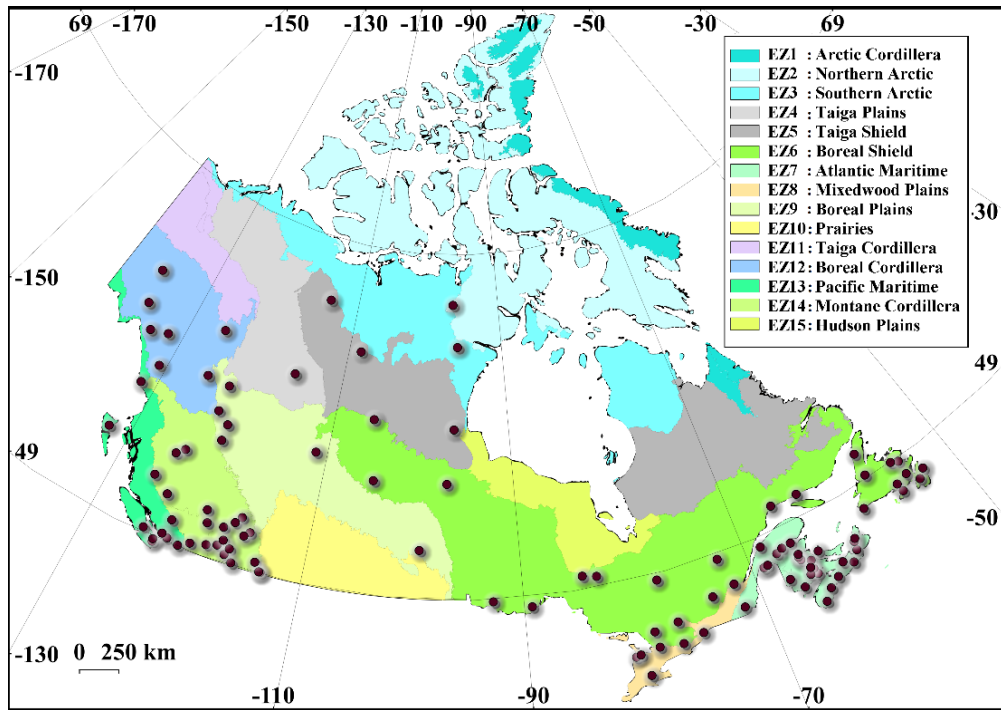
Figure 5 The distribution of the selected 105 RHBN streamflow stations within the Canadian ecoregions.
