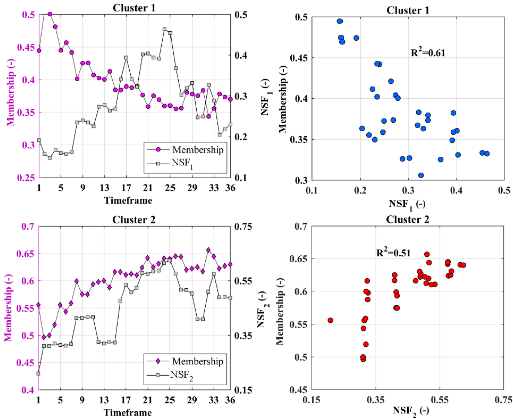
200 Figure 3. The procedure of attributing changes in membership degrees to changes in streamflow characteristics. The left column shows the co-evolution of membership degrees and Normalized Streamflow Features (i.e., NSF_1 and NSF_2 ). The right column measures the correspondence between changes in membership degrees and normalized streamflow features through percentage of described variance quantified using R^2 . Red or blue dots show the positive or negative dependencies, respectively.
