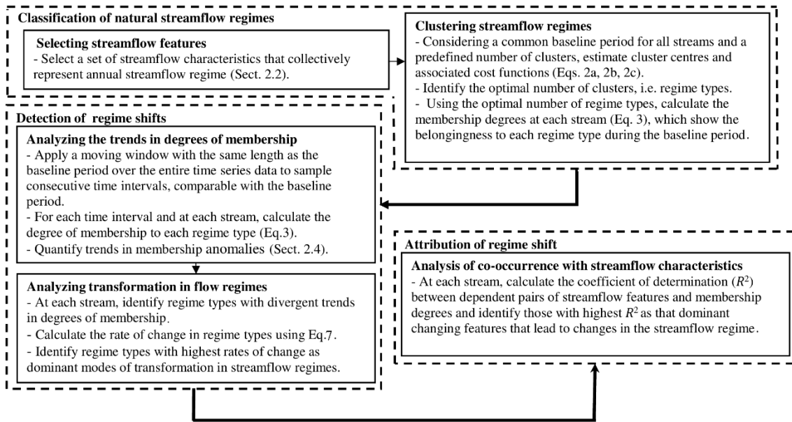
95 Figure 1. The workflow of the proposed three-step algorithm for classifying streamflow regime, diagnosing shift in streamflow regime, and attributing the regime shift to the changes in streamflow characteristics.
