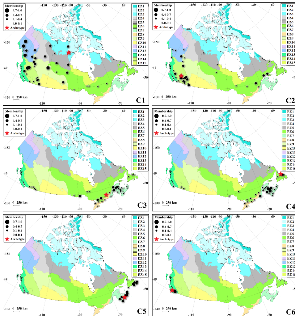
340 Figure 6. The distribution of the identified regime types across Canadian eozones during the baseline I timeframe of 1966 to 1975. Each stream is represented by a circle with a radius proportional to a membership degree quantifying the association to a given regime type. Only RHBN stations with degrees of membership of 0.1 or larger are shown in each panel. The red stars are the archetype stations related to each regime type.
