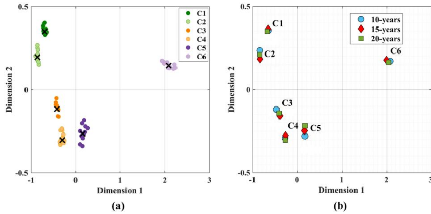
490 Figure 10. The sensitivity of the cluster centers to (a) the choice of decadal timeframe for clustering, and (b) the length of the timeframe used for analysis. In panel (a) dots show the two dimensional scaling of the cluster centers in which distances between dots represent dissimilarities between cluster centers. Black crosses show the centers identified by choosing the first decadal timeframe. Panel (b) shows the two dimensional scaling of the cluster centers considering 10-, 15- and 20-year timeframes.
