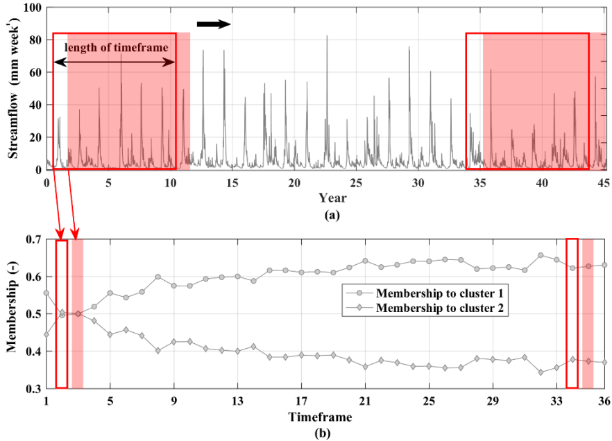
Figure 2. A schematic view to the procedure of identifying the evolution in membership values using a moving window; (a) a decadal timeframe slides over the streamflow time series year-by-year; (b) membership degrees are recalculated at each decadal timeframe to systematically determine the changes in association to each regime type determined in the beginning of the data period.
