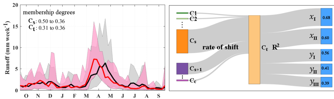
220 Figure 4. An example for transitions between regime types along with attribution of change to streamflow characteristics. The left panel shows annual hydrographs in two separate periods using grey and pink envelopes. The panel in the right shows the dominant shift in the flow regime by maximum rate of shift, and attributes this shift to changes in significantly dependent streamflow characteristics. The dominant shift is visualized by the thickest grey envelope. The strength of the association between regime shift and significantly dependent streamflow characteristics are measured and communicated by R^2 .
