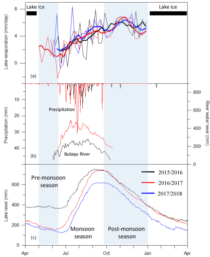
710 Figure 7: The main components of lake water budget at Paiku Co between 2015 and 2018. (a): Lake evaporation (mm/day) derived from the north shoreline of Paiku Co. (b): Daily precipitation (mm) at Qomolangma station and water level (mm) of Bulaqu River in 2015 and 2016. Note the Y axis (left) of precipitation is reversed. (c): Daily lake level (mm) at Paiku Co. The thick lines (a) denote the 5-point running average. The blue rectangles represent pre-monsoon and post-monsoon seasons periods, respectively.
