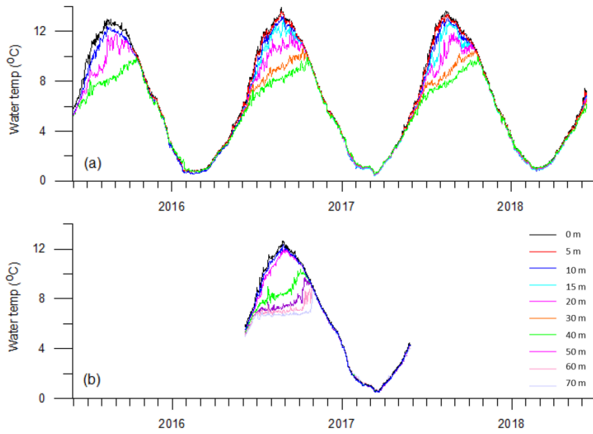
Figure 2: Time series of daily lake water temperature at different water depths in Paiku Co's southern (a) and northern basins.
