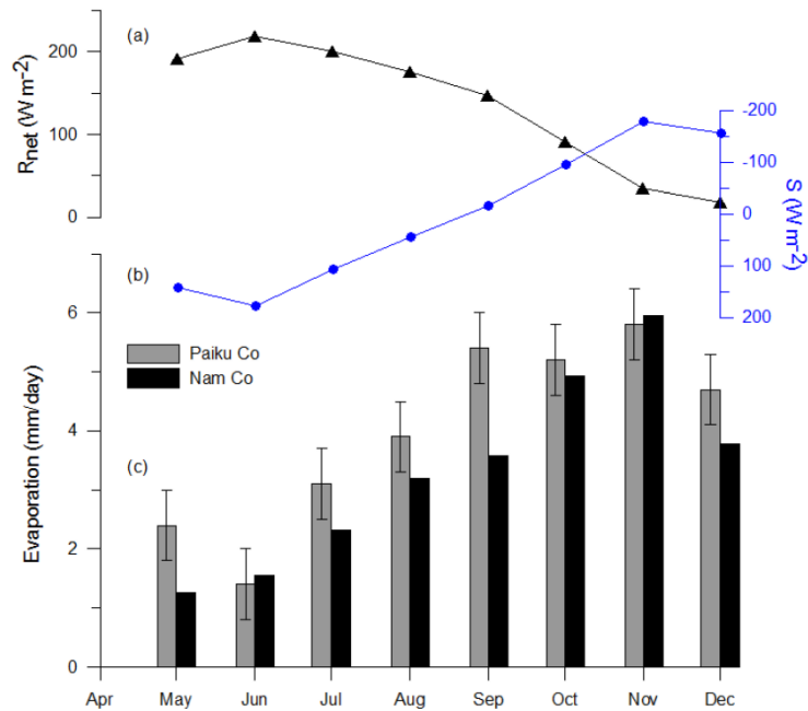
Fig. 6 A Comparison of monthly lake evaporation with net radiation ( R_{net} ) and changes in lake heat storage ( S ). (a): Net radiation, (b): Changes in lake heat storage, (c): Lake evaporation from Paiku Co and Nam Co on the central TP.
