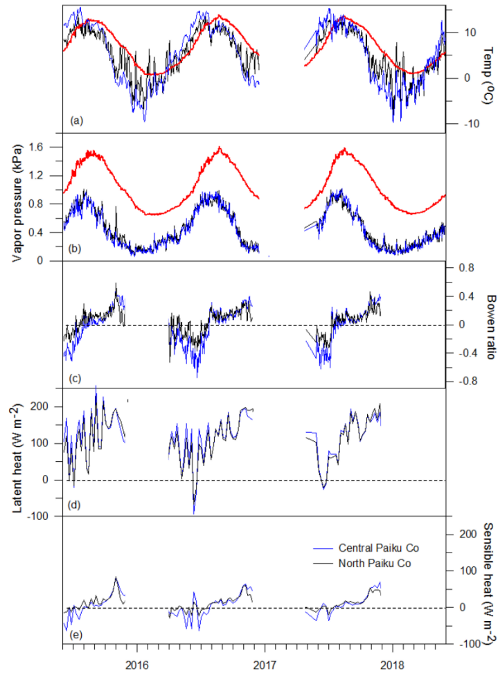
675 Figure 5: Hydrometeorology and heat fluxes at the lake surface. (a): Daily air temperature and lake surface temperature (red line), (b): Daily actual vapour pressure at lake surface (red line) and the overlying atmosphere, (c): Daily Bowen ratio between May and December, (d-e): Weekly averaged latent and sensible heat fluxes between May and December. For a-e, black lines denote north Paiku Co and blue lines denote central Paiku Co. There was no data available between February and May 2017.
