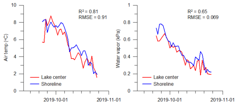
740 Figure 9: Comparison of daily air temperature and water vapour pressure between shoreline and lake centre during the period of 23/9/2019-25/10/2019.
