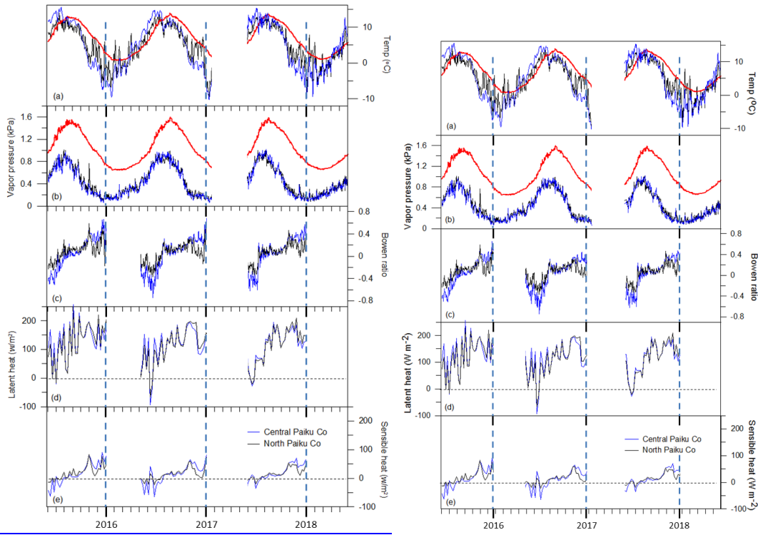
Figure 5: Hydrometeorology and heat fluxes at the lake surface. (a): Daily air temperature and lake surface temperature (red line), (b): Daily actual vapour pressure at lake surface (red line) and the overlying atmosphere, (c): Daily Bowen ratio between May and December, (d-e): Weekly averaged latent and sensible heat fluxes between May and December. For a-e, black lines denote north Paiku Co and blue lines denote central Paiku Co. There was no data available between February and May 2017.
