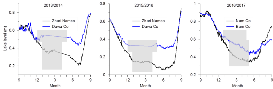
775 Figure 8: Different amplitude of seasonal lake-level changes between deep and shallow lakes on the central TP. Relatively deep lakes: Zhari Namco (85.61 °E, 30.93 °N) and Nam Co (90.60 °E, 30.74 °N); Relatively shallow lakes: Dawa Co (84.96 °E, 31.24 °N) and Bam Co (90.58 °E, 31.26 °N). Grey rectangles in each figure represent lake ice covered periods.
