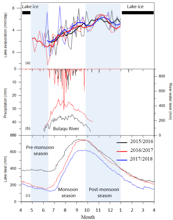
765 Figure 7: The main components of lake water budget at Paiku Co between 2015 and 2018. (a): Lake evaporation (mm/day) derived from the north shoreline of Paiku Co. (b): Daily precipitation (mm) at Qomolangma station and water level (mm) of Bulaqu River in 2015 and 2016. Note the Y axis (left) of precipitation is reversed. (c): Daily lake level (mm) at Paiku Co. The thick lines (a) denote the 5-point running average. The blue rectangles represent pre-monsoon and post-monsoon seasons periods, respectively.
