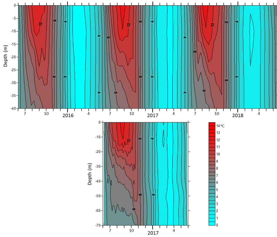
730 Figure 3: Depth-time diagram of isotherm (°C) in Paiku Co's southern (upper, 42 m in depth) and northern (below, 72 m in depth) basins between June 2015 and May 2018.
