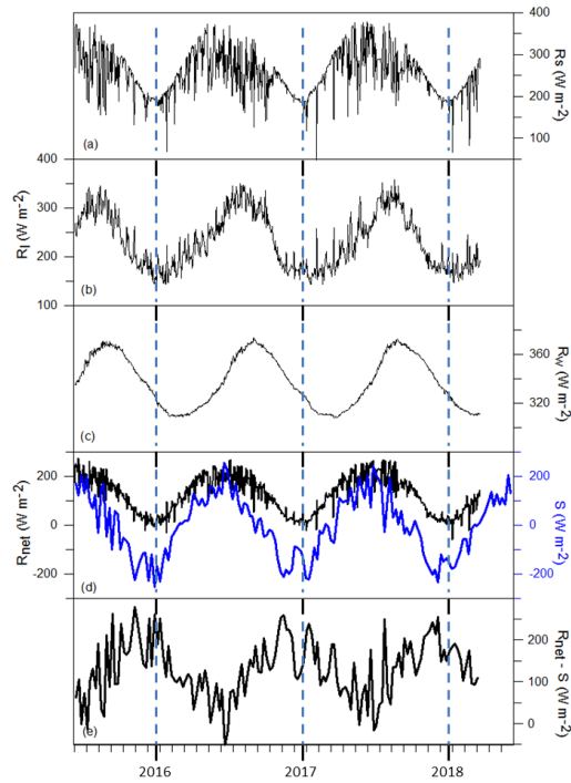
735 Figure 4: The main components of energy budget at the lake surface. (a): Daily solar radiation ( R_s ), (b): Daily atmospheric longwave radiation to the lake ( R_a ), (c): Daily long wave radiation emitted from the lake ( R_w ), (d): Daily net radiation ( R_{net} ) and weekly changes in lake heat storage ( S ), (e): The available energy (Weekly changes in lake heat storage) ( R_{net}-S ).
