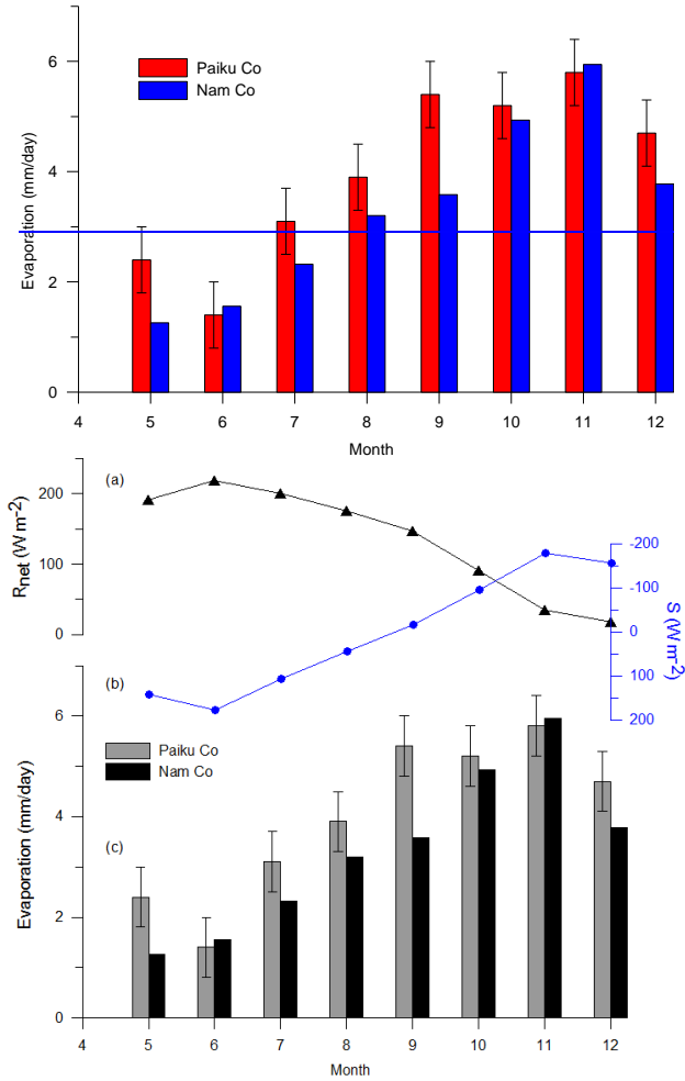
Fig. 6 A Comparison of monthly lake evaporation with net radiation ( R_{net} ) and changes in lake heat storage ( S ). (a): Net radiation, (b): Changes in lake heat storage, (c): Lake evaporation at Paiku Co with and Nam Co on the central TP. Lake evaporation at Nam Co was determined by using eddy covariance system in the lake center (Wang et al., 2019). The bars denote the uncertainty of lake evaporation at Paiku Co.
