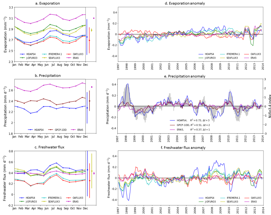
Figure 3. Climatological (1997–2013) seasonal cycle of global ocean mean evaporation rate (a), precipitation rate (b), and freshwater flux (c). HOAPS, ERA5, OAFflux, SEAFLUX, and GPCP mean values and associated 1\sigma uncertainty ranges are shown in the boxes to the right of the panels. Monthly mean anomaly (w.r.t. the climatological seasonal cycle depicted at left) over the global oceans ( 80^\circ S– 80^\circ N) of evaporation rate (d), precipitation rate (e), and freshwater flux (f). The anomaly data are smoothed using a three-month running mean. Panel e additionally displays the Niño3.4 index shifted by +3 months (right y-axis). The legend shows the correlation coefficient of the Niño3.4 index with P anomalies and the time lag of highest correlation ( \Delta t in months). Ticks on the time axis mark January of the indicated year.
