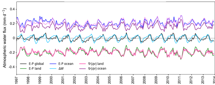
Figure 7. ERA5 monthly mean E - P over the whole globe (black), land only (green), and ocean (blue); global mean \Delta W (light blue), mean \nabla \cdot (vq) over land (pink) and ocean (purple). The mean values over the globe and land were scaled by their surface area relative to the ocean surface area (i.e., they were multiplied by 510/350 and 160/350 , respectively) to obtain consistency with the over-ocean means shown in Fig. 3. Error bars represent the standard deviation within the 10-member ensemble, which is smaller than the graph's line width for E - P over land, \Delta W , and \nabla \cdot (vq) .
