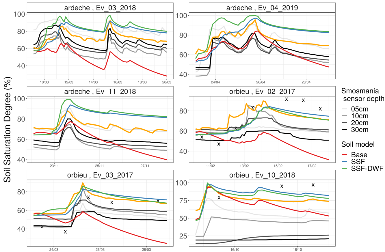
Figure 5. SMOSMANIA SSD measurement at the four sensor depths for the Barnas (Ardeche catchment) and the Mouthoumet (Orbieu catchment) stations, together with the SSD simulated with MARINE, the LDAS-Monde HU_{surf} and the CGLS SWI when available at the measurement point location. For the MARINE simulations using the SSF-DWF soil model, the moisture of the surface layer is considered here.
