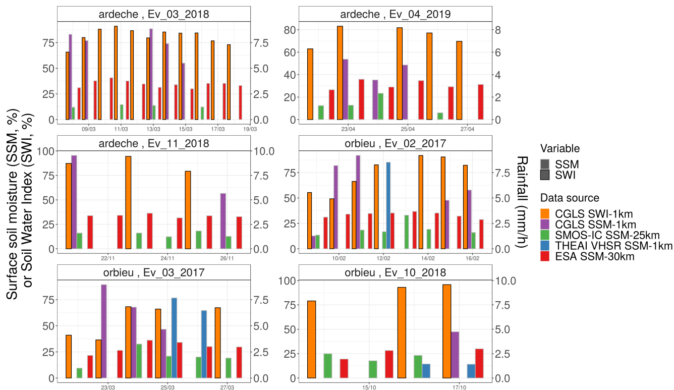
Figure A1. Daily values of Surface soil moisture (SSM) or Soil Water Index (SWI) provided by the CGLS, SMOS-IC, THEIA-Land VHSR and ESA CCI products (left axis), along with associated ANTILOPE precipitation (right axis), on average over the two studied catchments during the six simulated events.
