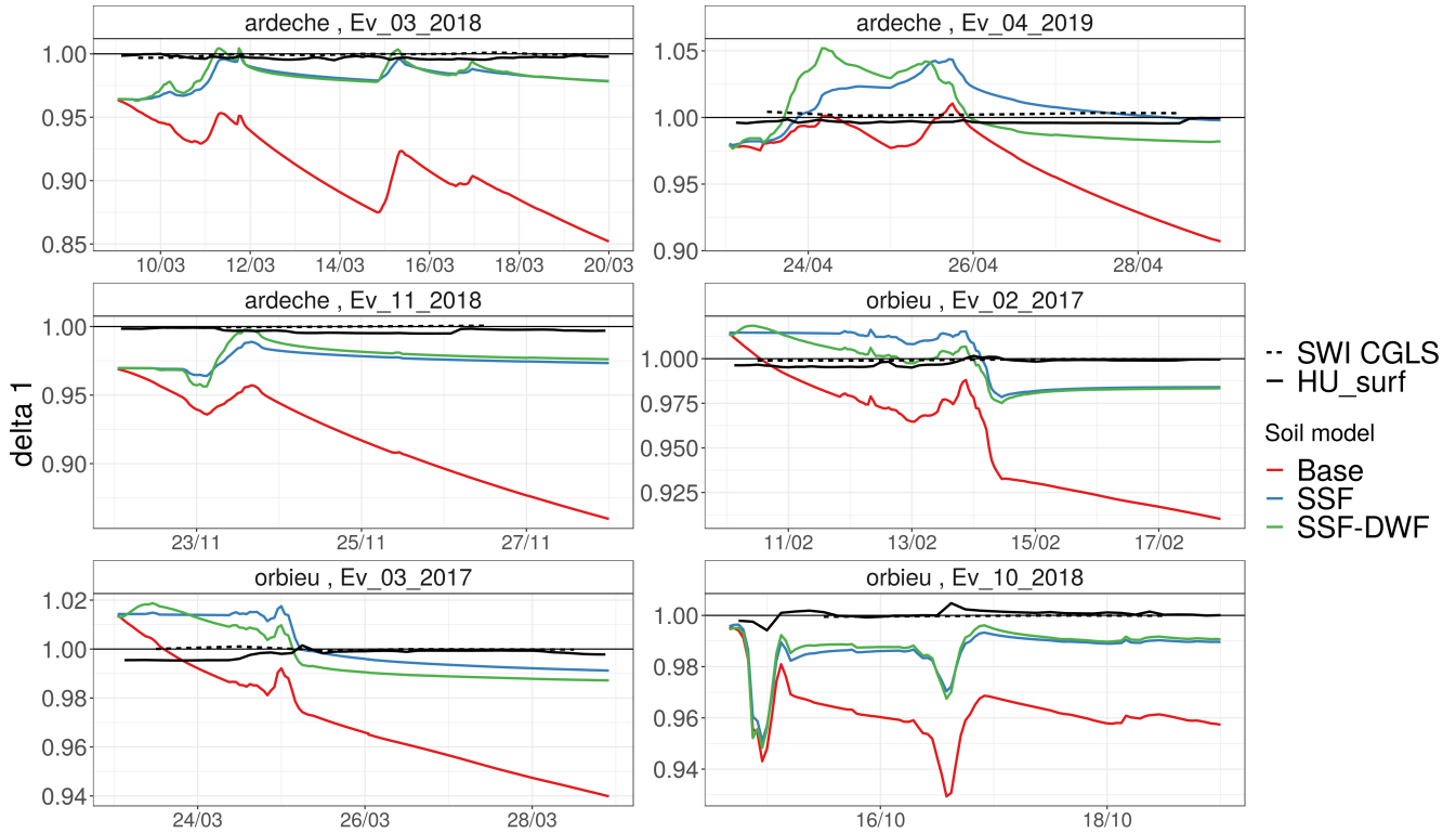
Figure 8. Time series of index \delta 1 defined by Zocatelli et al. (2011) for the six events, computed for the SSD outputs for the BM, SSF and SSF-DWF models, and also for the LDAS-Monde HU_{surf} variable and the CGLS SWI.
