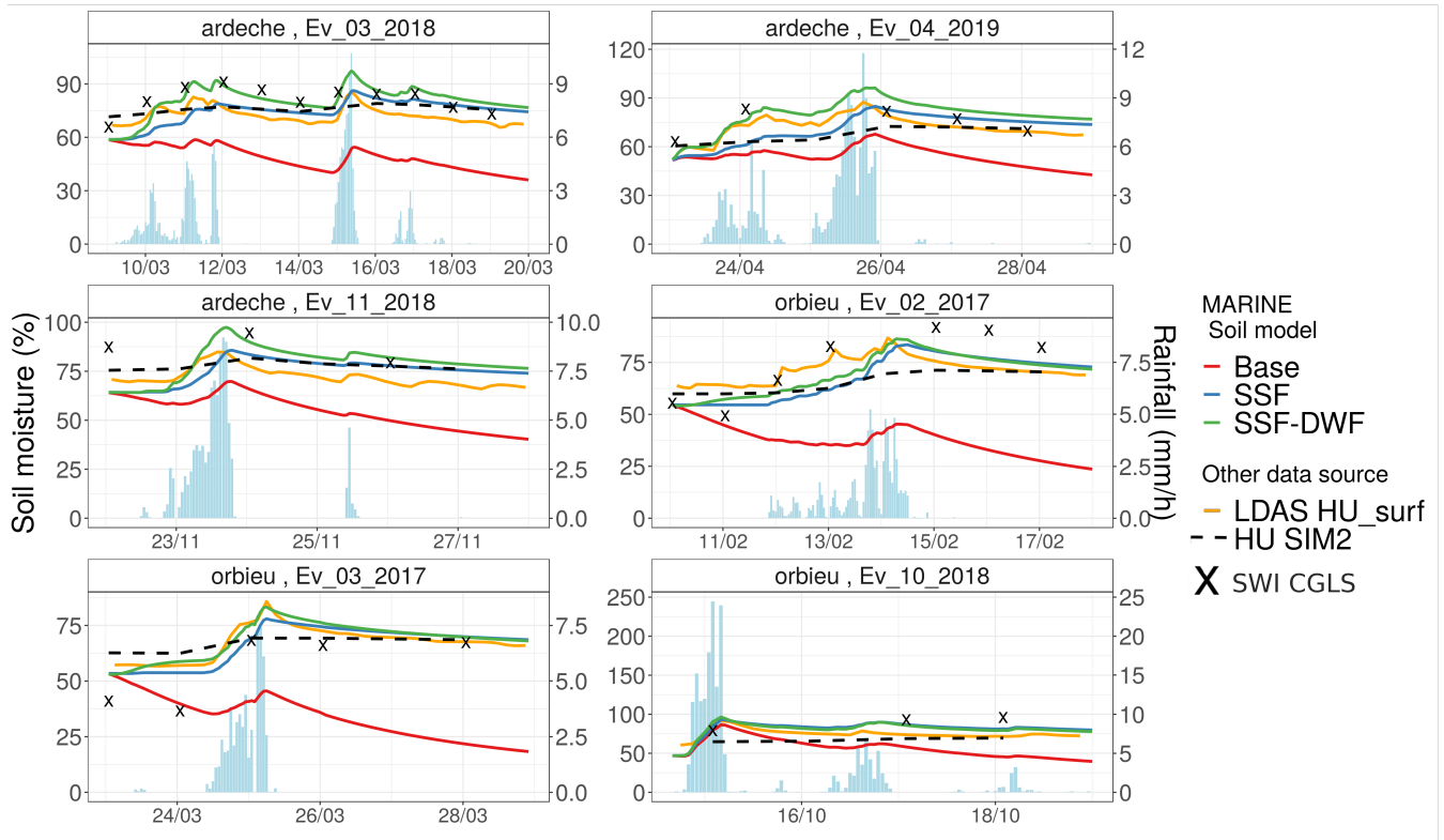
Figure 6. SSD time series, on average per catchment, simulated with MARINE using the base, the SSF or the SSF-DWF models, and LDAS-Monde HU_{surf} and SWI CGLS values, in average per catchment.
