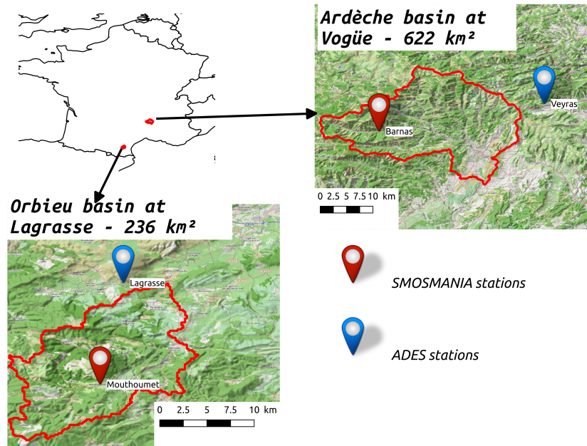
Figure 2. The two studied catchments located in the South of France: the Ardeche river at Vogue and the Orbieu river at Lagrasse. Monitoring networks: soil water content (SMOSMANIA network stations) and the national groundwater ADES network stations ( www.adeseaufrance.fr ).
