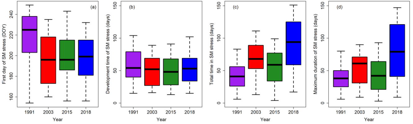
350 Figure 8. Variability of different SM stress characteristics shown for the prominent drought years. Shown are (a) first day ( S_{\text{start}} ), (b) development time ( S_{\text{devtime}} ) (c) total number of days ( S_{\text{total}} ), and (d) maximum duration ( S_{\text{maxdur}} ) of SM stress. Box: percentiles 25, 50 and 75. End of whiskers: percentiles 5 and 95.
