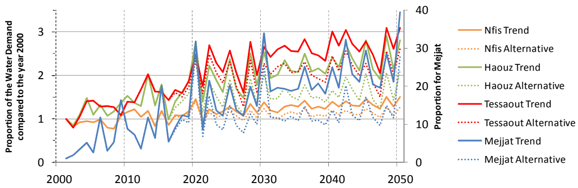
Figure 7: Trend and alternative scenarios for irrigation-water demand in the four planning areas of the Tensift with RCP8.5.
