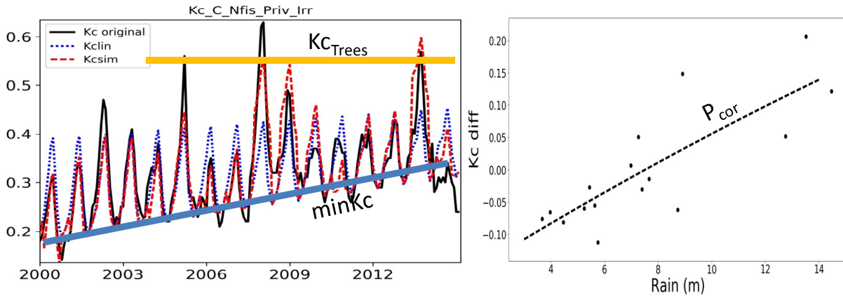
580 Figure 3: Quantities used to perform the simulation. The example illustration on the left depicts the synthetic K_c of the N'Fis private area where a mix of tree crops (olive, orange, apricot) and cereals crop (mainly wheat) are cultivated. The peak occurs during March/April when cereal crops are at their maximum development, the valleys correspond to the summer months when there are no seasonal crops. The three curves are the K_c time series obtained from remote sensing processing (solid line), the linear estimation ( K_{clin} , Eq. 3, dotted blue line) and the estimation corrected with rainfall ( K_{csim} , Eq. 6, dashed red line). K_{cTrees} has been set to 0.55 in Eq. 8, and minK_c is the yearly minimum of K_c on K_{csim} . On the right, the fitted correction curve of K_c according to the cumulated rainfalls ( P_{corr} ) is almost linear in this example.
