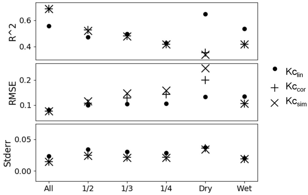
Figure 4: Performance indicators ( r^2 , RMSE, stderr) for the three variations of the model ( Kc_{lin} , Kc_{cor} , Kc_{sim} ) as a function of the splitting strategy for determining the calibration/validation data set.
