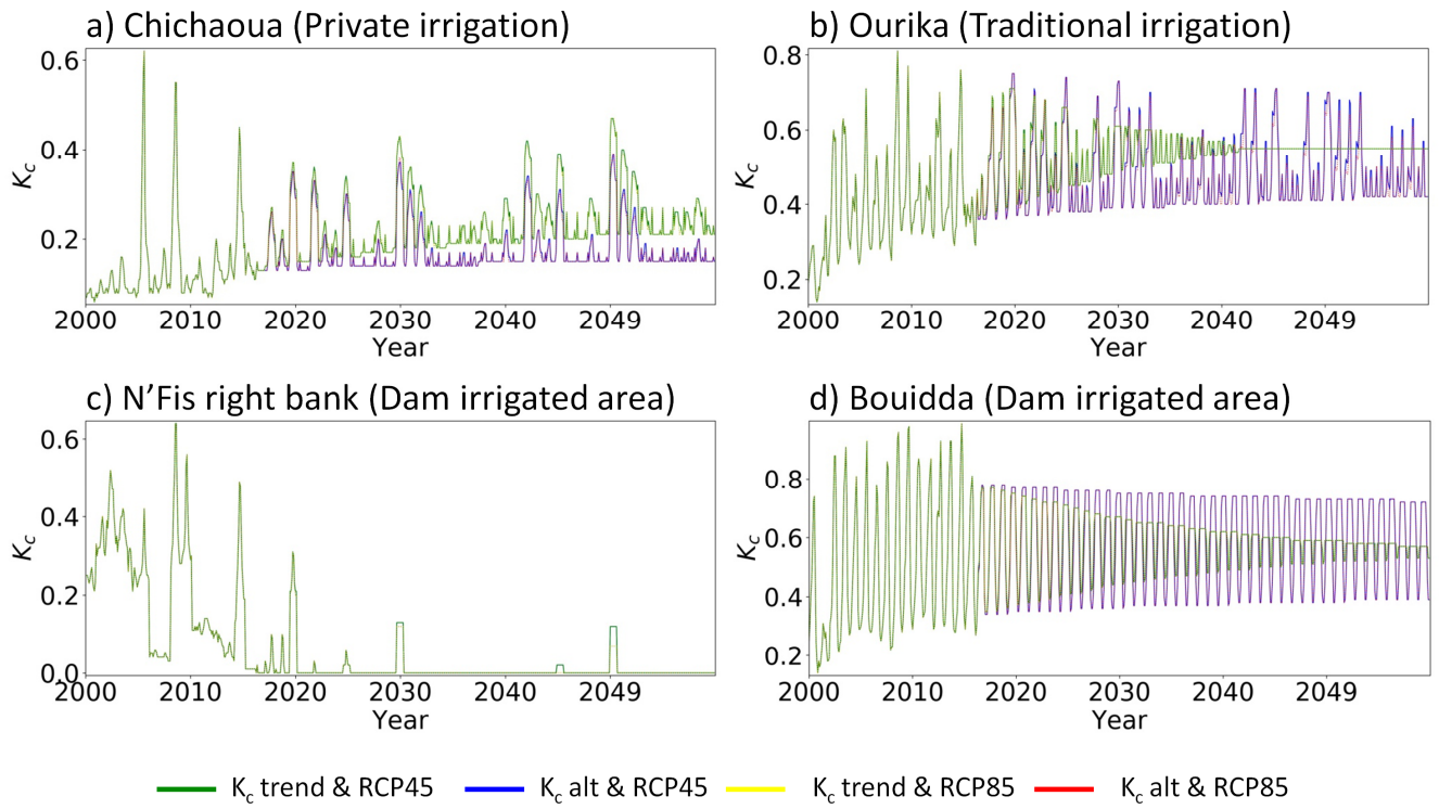
595 Figure 6: Examples of long-term simulation of K_c in four different irrigated areas with the trend and alternative scenarios of K_c and the RCP4.5 and RCP8.5 climatic scenarios.
