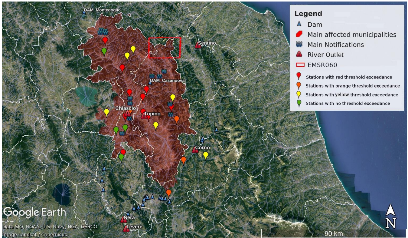
1360 Figure 2: geo-referred information of ODB for CS01, Umbria Region, with localization of main recorded floods (blue waves), hydrometric stations used for the indices validation (pinpoints). Red triangles indicate the position of outlets of main involved rivers, while blue triangles indicates the presence of dams. Hydrometric station pinpoints are coloured according to the maximum hydrometric threshold reached during the event. Municipalities areas affected by floodings are filled in red. Red rectangle represents the involved area published on COPERNICUS Emergency Management Service Platform ( https://emergency.copernicus.eu/mapping/list-of-components/EMSR060 ).
