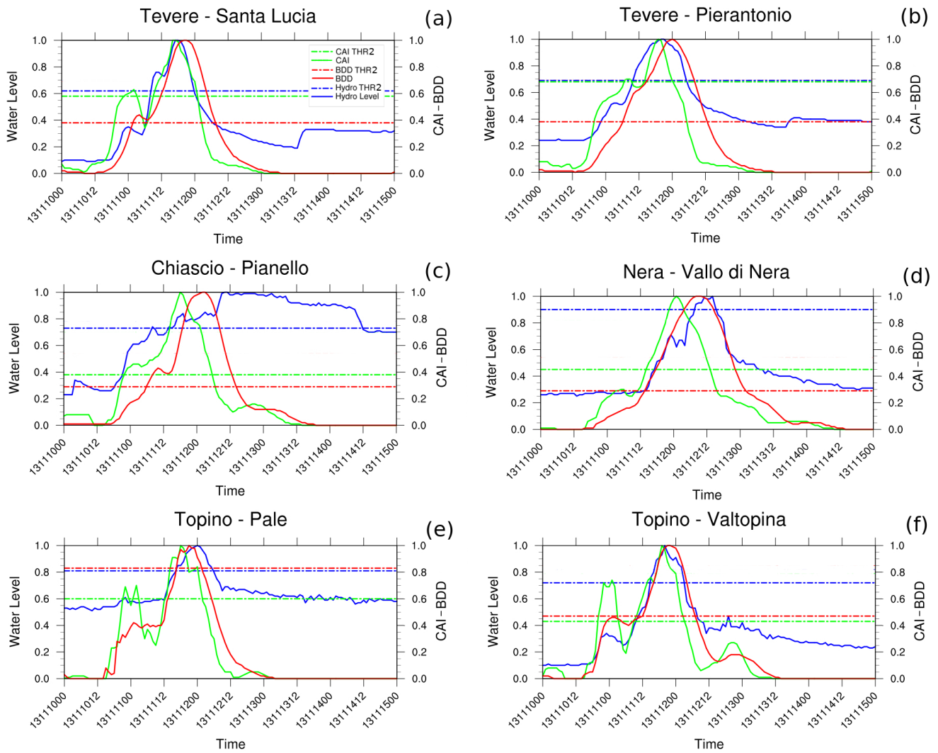
1415 Figure 9: time series comparison for six hydrometric stations: BDD hourly profile (red line), BDD Moderate Threshold (red flat line); CAI hourly profile (green line), CAI Moderate Threshold (green flat line); Hydrometric Level hourly profile (blue line), Hydrometric Level Moderate Threshold (blue flat line). Quantities profiles and related thresholds are normalized.
