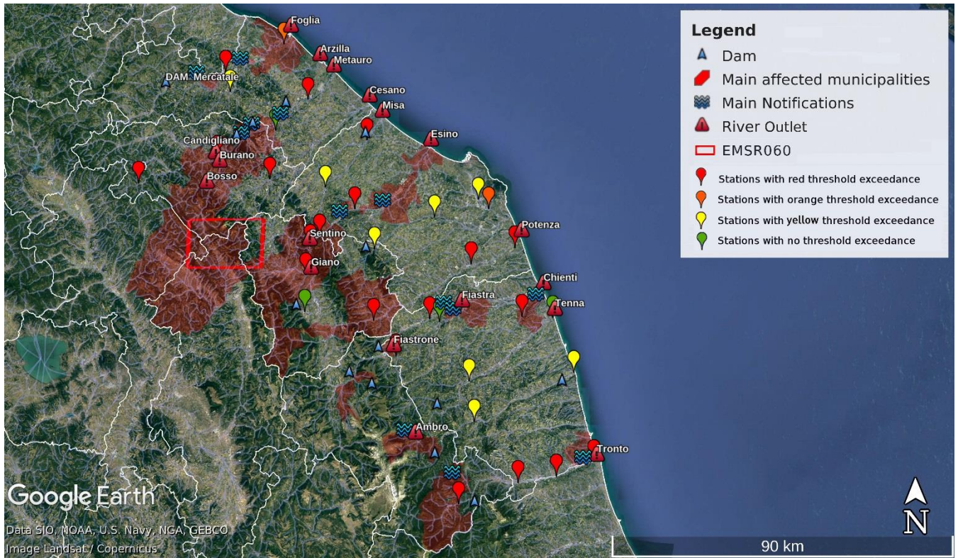
1370 Figure 3: geo-referred information of ODB for CS02, Marche Region, with localization of main recorded floods (blue waves), hydrometric stations used for the indices validation (pinpoints). Red triangles indicate the position of outlets of main involved rivers, while blue triangles indicates the presence of dams. Hydrometric station pinpoints are coloured according to the maximum hydrometric threshold reached during the event. Municipalities areas affected by floodings are filled in red.
