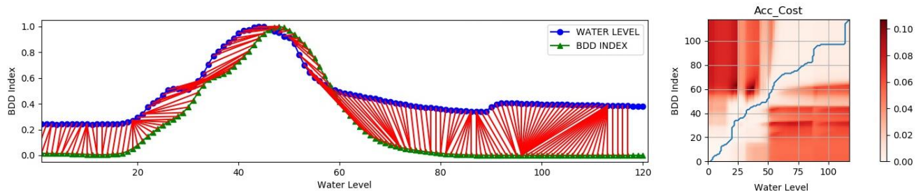
1390 Figure 5: graphical representation of DDTW correspondences between two first derivatives of time series x(t) and y(t) . In this case, time series are represented by two generic profiles of the hydrometric water level and the BDD index, at the same station point (from Keogh and Pazzani, 2001).
