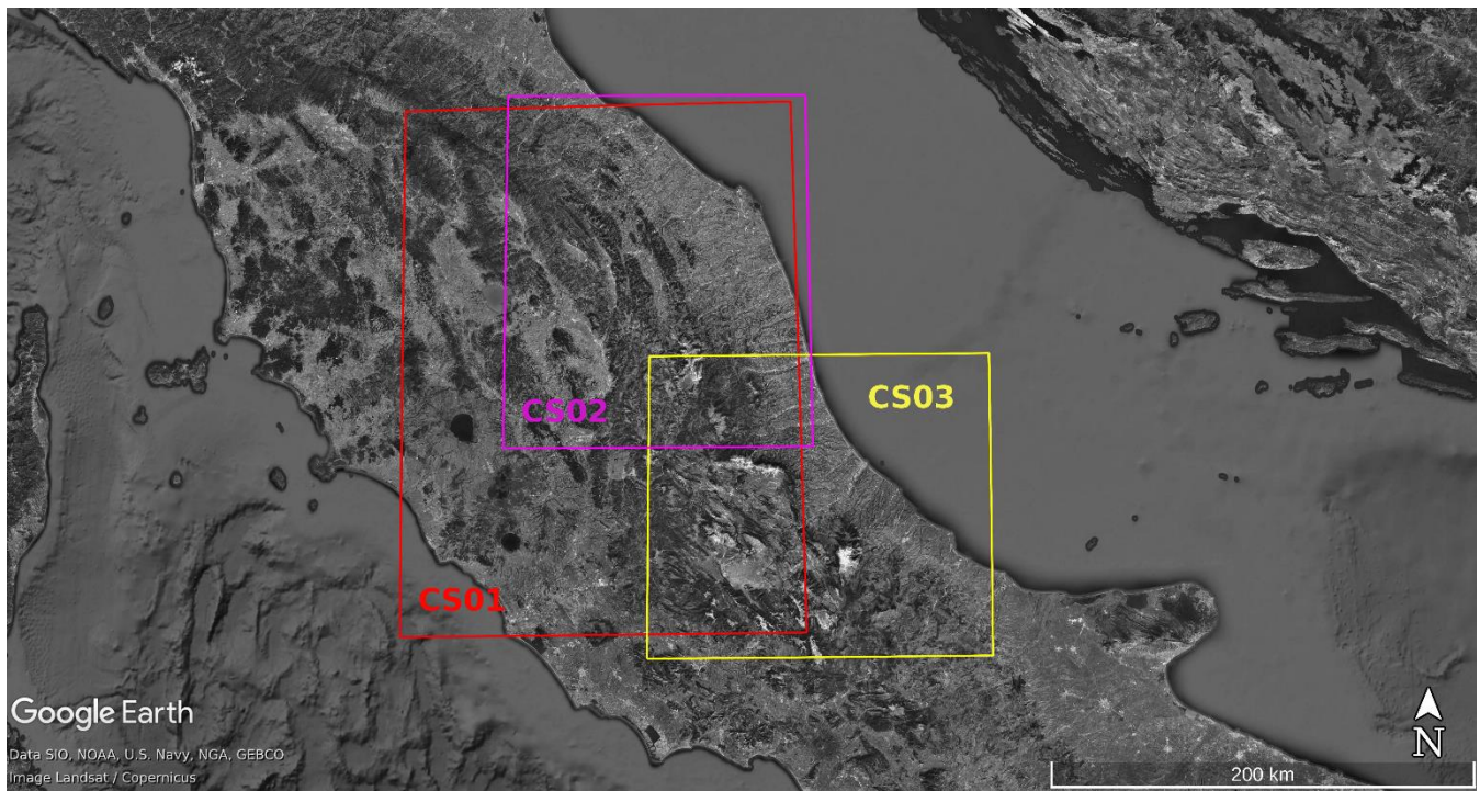
Figure 6: three CHyM geographical domains used for the simulation of the corresponding CSs. The red square encloses Umbria Region and the rest of Tiber basin for CS01, pink square refers to CS02 (Marche Region) and yellow square encompasses Abruzzo Region for CS03.
