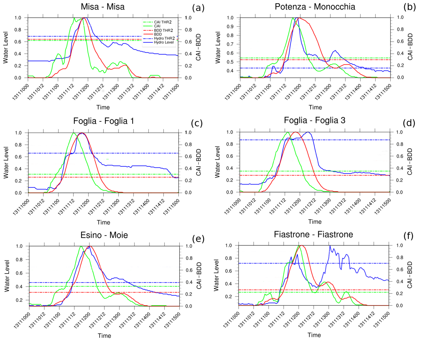
1430 Figure 13: time series comparison for six hydrometric stations: BDD hourly profile (red line), BDD Moderate Threshold (red flat line); CAI hourly profile (green line), CAI Moderate Threshold (green flat line); Hydrometric Level hourly profile (blue line), Hydrometric Level Moderate Threshold (blue flat line). Quantities profiles and related thresholds are normalized.
