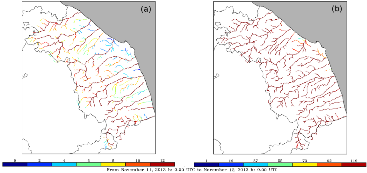
Figure 10: CS02 24 hours maps of BDD index (left) and CAI index (right) obtained for November 11th 2013, by forcing the CHyM model with observed rainfall data. Warmer colours indicate river segments with higher flood stress. In both figure, the Marche region drainage network is highlighted
