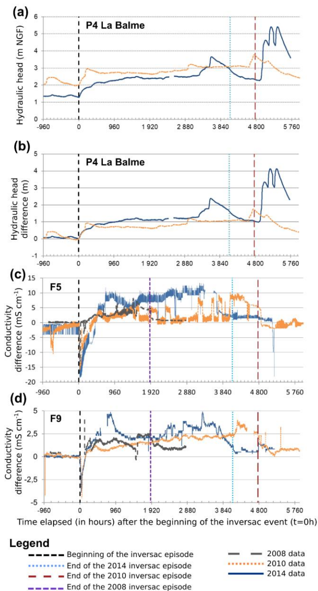
Figure 5 (a) Hydraulic head (m) and (b) hydraulic head variation (m) of the karst well P4 La Balme during the 2010 and 2014 inversac events; electrical conductivity variation ( \text{mS cm}^{-1} ) for the thermal wells (c) F5 and (d) F9 during the 2008, 2010 and 2014 inversac events.
