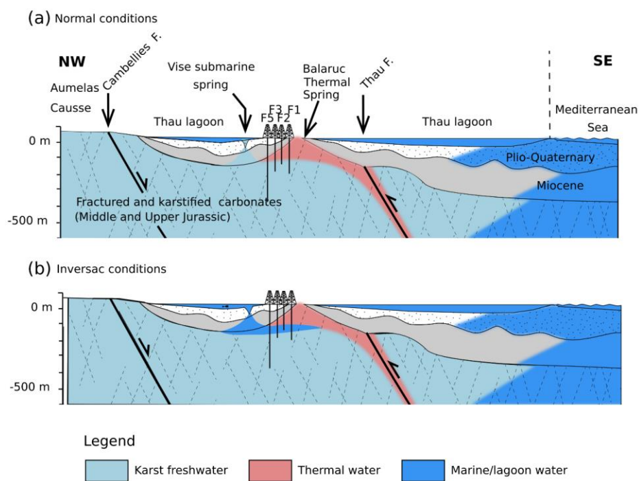
294 Figure 2: Conceptual cross-section oriented NW-SE passing through thermal wells of the Balaruc peninsula, and 295 showing groundwater flows of the karst hydrosystem under (a) normal conditions and (b) inversac conditions. 296 Location of the cross-section is indicated in Figure 1a.
