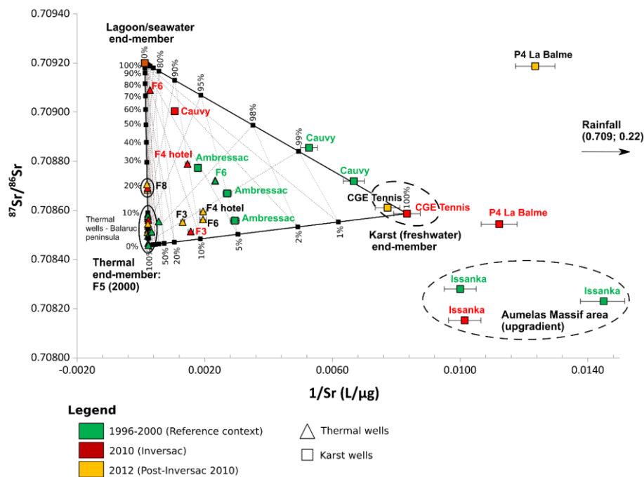
527 Figure 8 Plot of ^{87}\text{Sr}/^{86}\text{Sr} ratio versus Sr concentration (as 1/\text{Sr} ) for springs and wells of the Balaruc peninsula 528 for different hydrogeological situations: pre-inversac reference (green), 2010 inversac (red) and 2012 post- 529 inversac (yellow). 530
